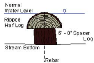
Section View
