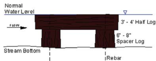
Profile View
