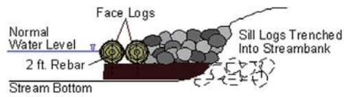
Section View
