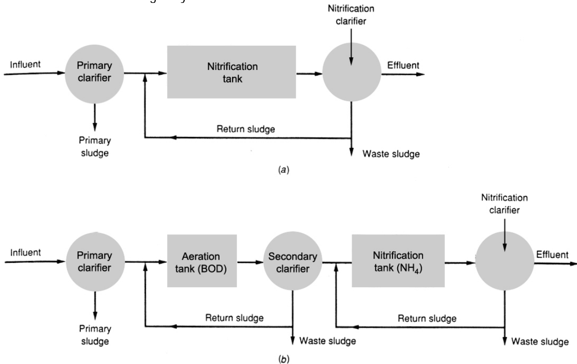
Figure 1.2 Single-stage and Separate-stage Biochemical Nitrification Processes 3
