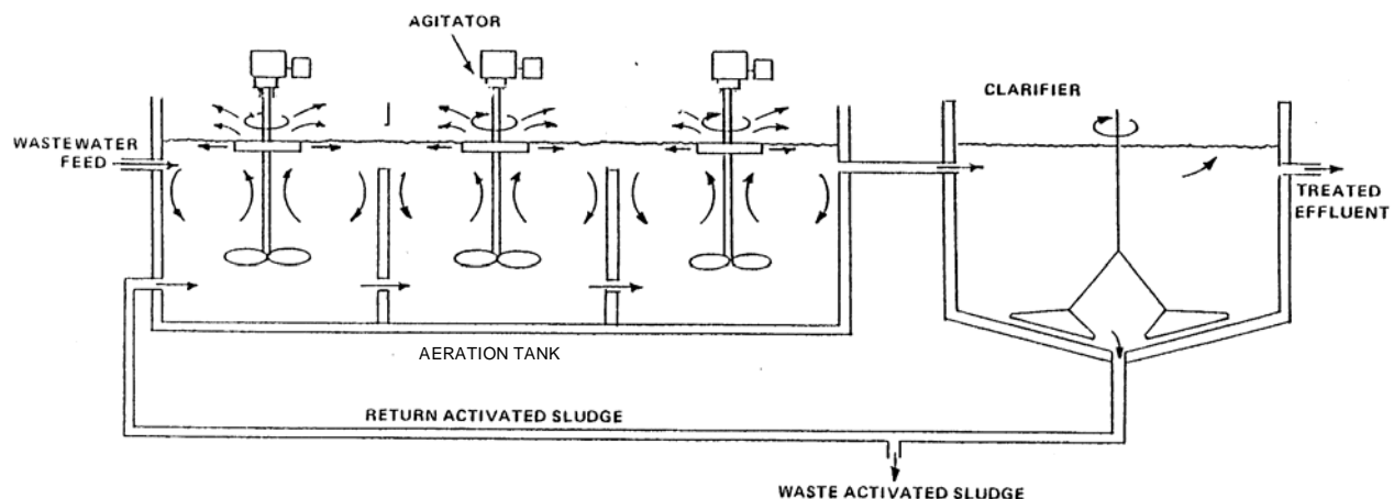
Figure 1.1 Diagram of aeration system in the activated sludge process 1
