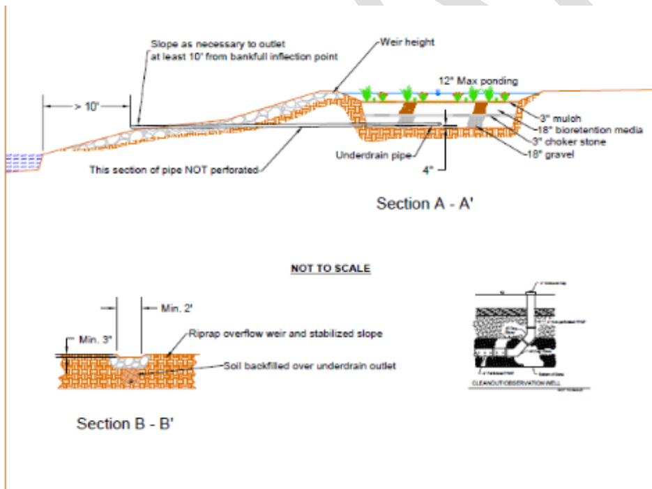
Figure B5: Bioretention Drawing
