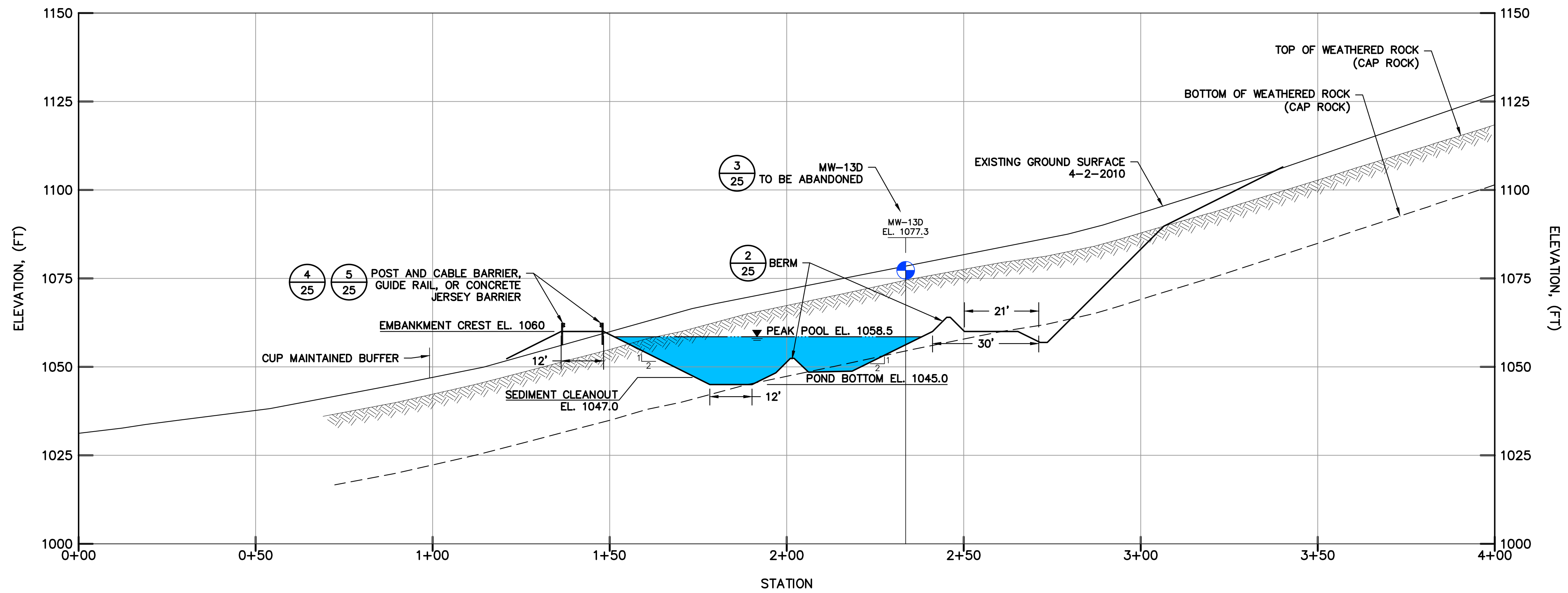
NT POND NO. 1 – SECTION B-B
