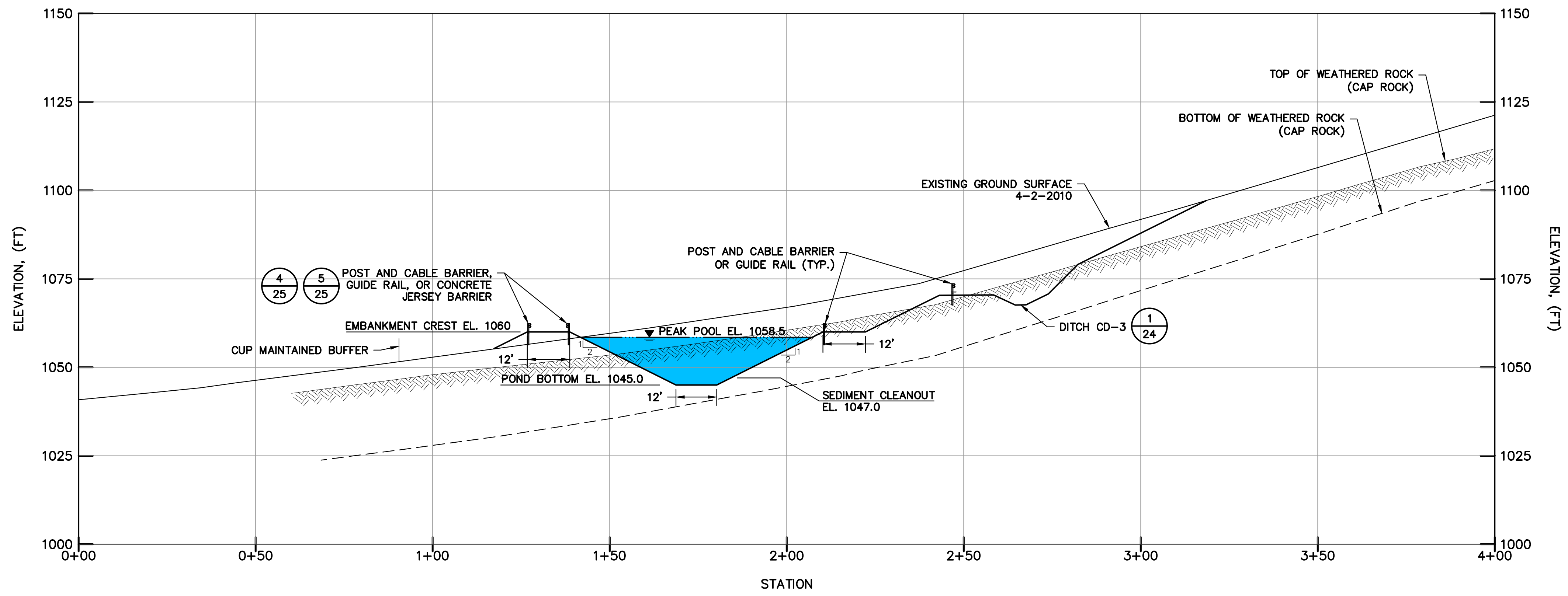
NT POND NO. 1 – SECTION A-A
