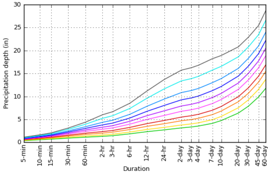
PDS-based depth-duration-frequency (DDF) curves Latitude: 39.7673°, Longitude: -77.4405°
