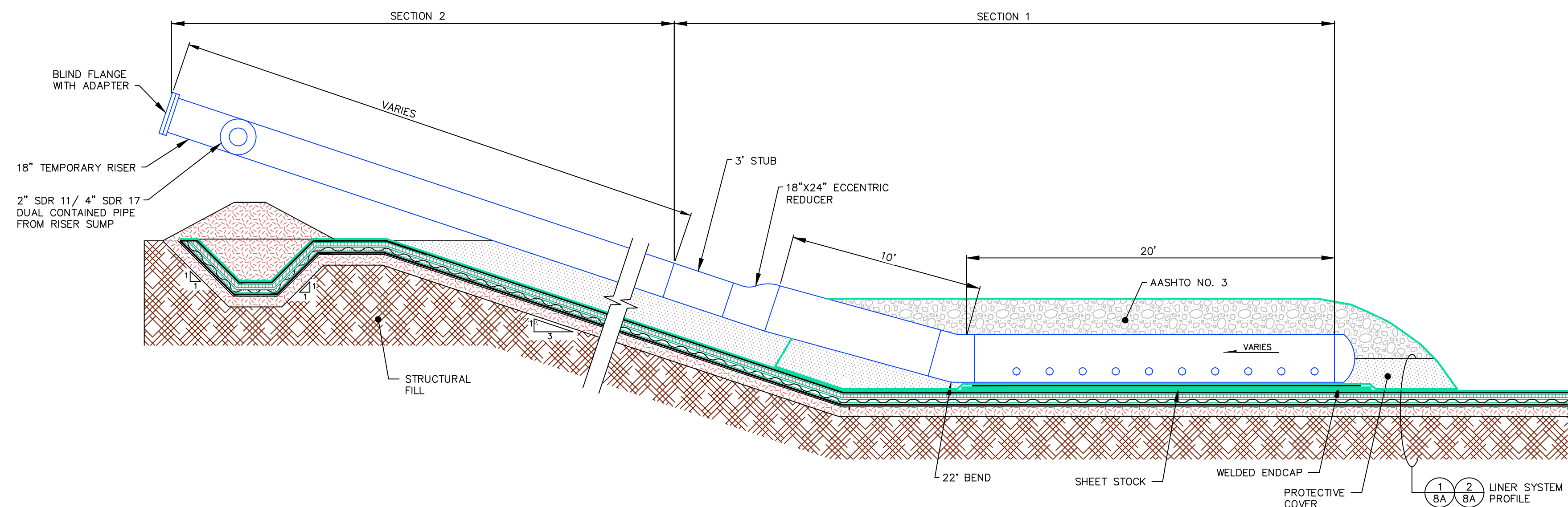
2 TEMPORARY SIDE SLOPE RISER DETAIL (SECTION A-A') BE NOT TO SCALE
