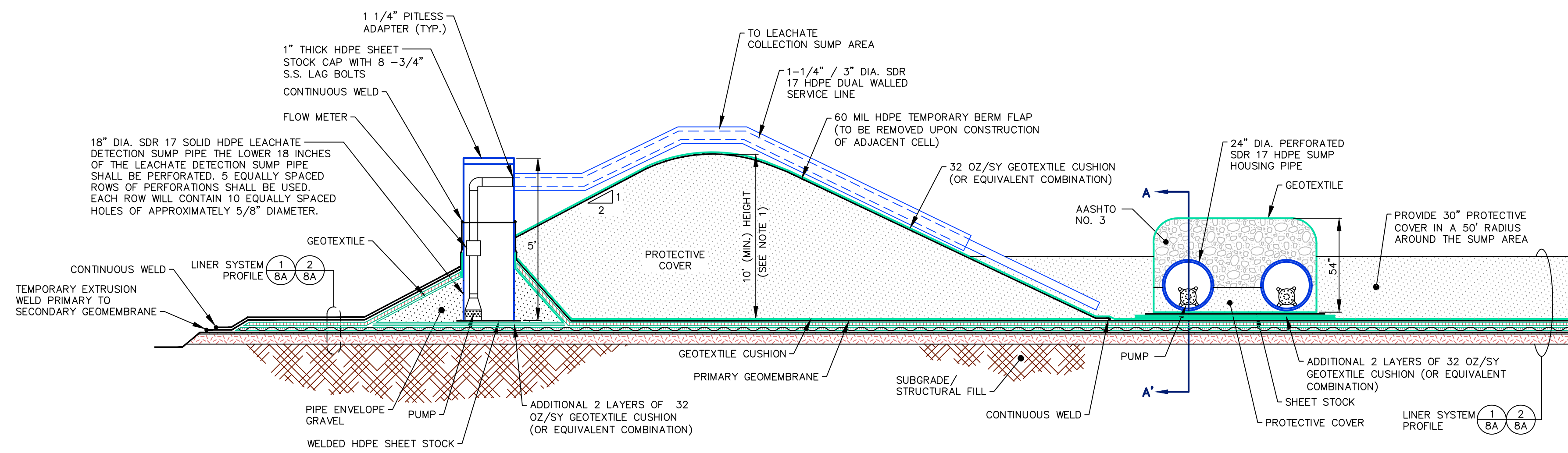
1 TEMPORARY LEACHATE COLLECTION / DETECTION SUMP BE NOT TO SCALE
