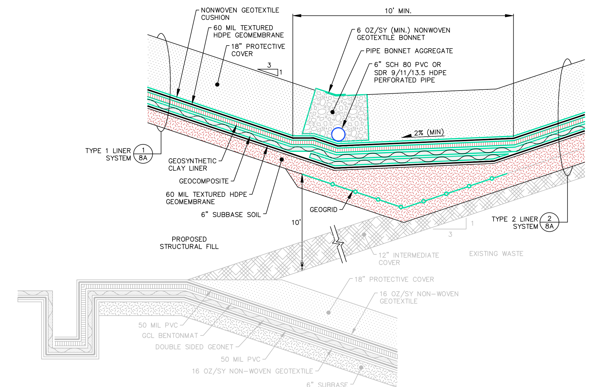
TYPE 4 LINER TERMINATION DETAIL 7 8A NOT TO SCALE
