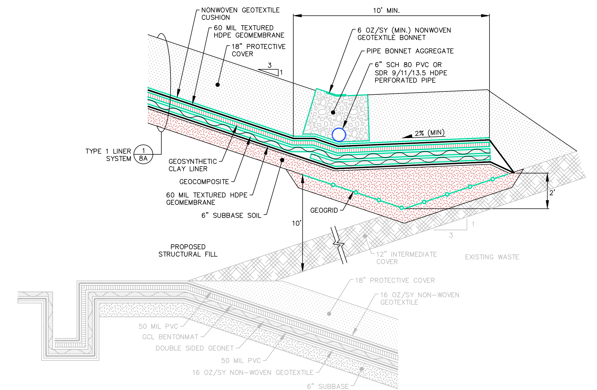
TYPE 2 LINER TERMINATION DETAIL 4 8A NOT TO SCALE
