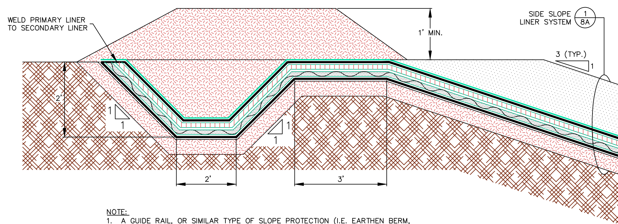
PERIMETER ANCHOR TRENCH DETAIL 5 8A NOT TO SCALE
