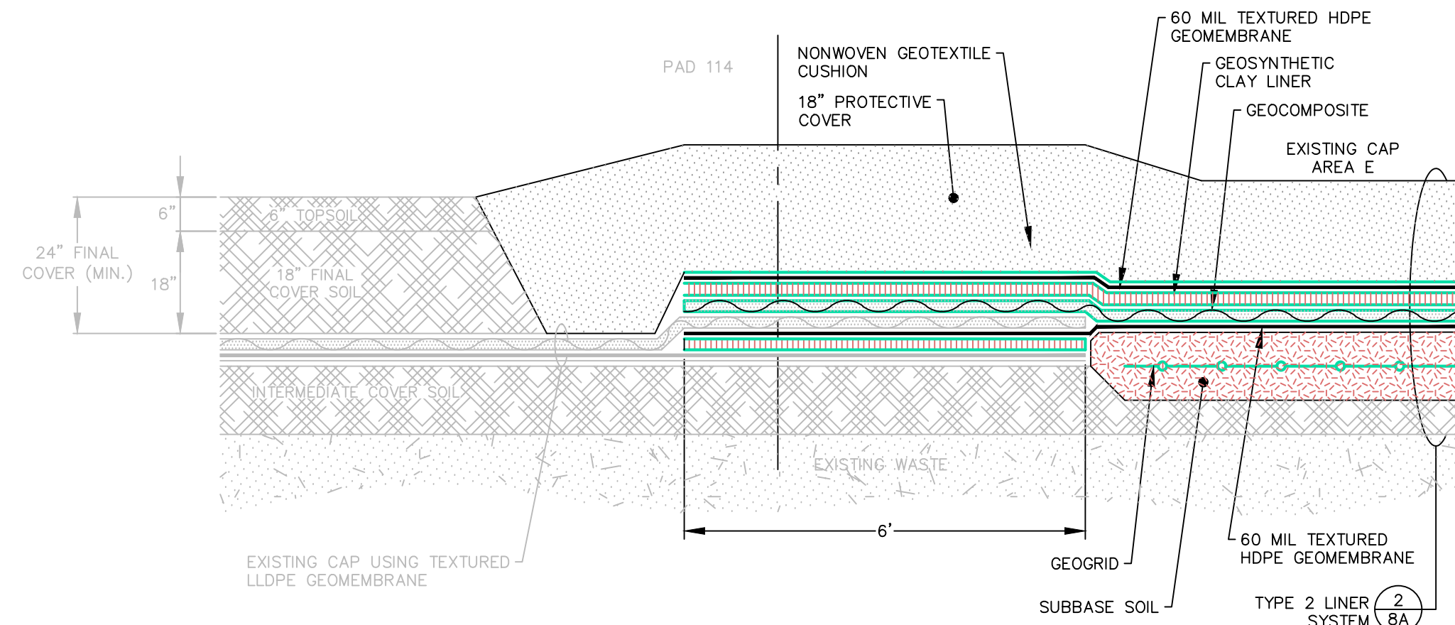
TYPE 3 LINER TERMINATION DETAIL 6 8A NOT TO SCALE
