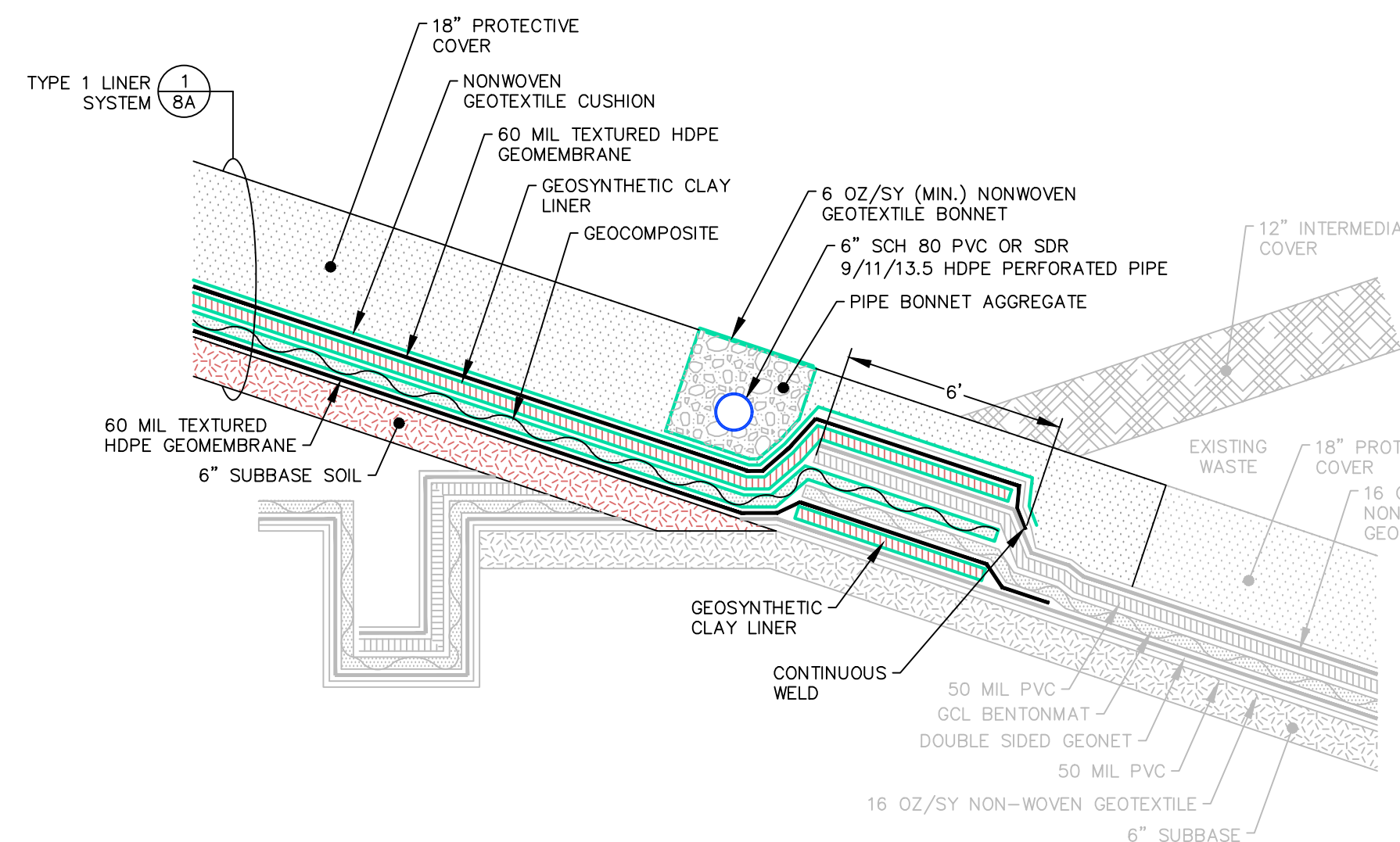
TYPE 1 LINER TERMINATION DETAIL 3 8A NOT TO SCALE
