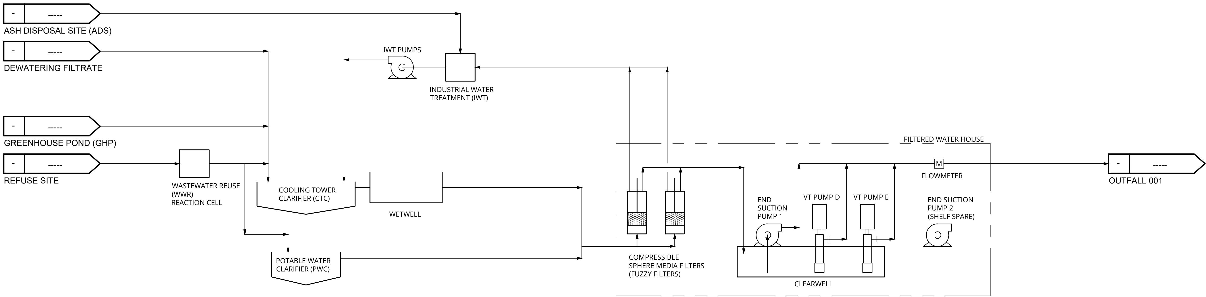
EXISTING SYSTEM WATER FLOW DIAGRAM
