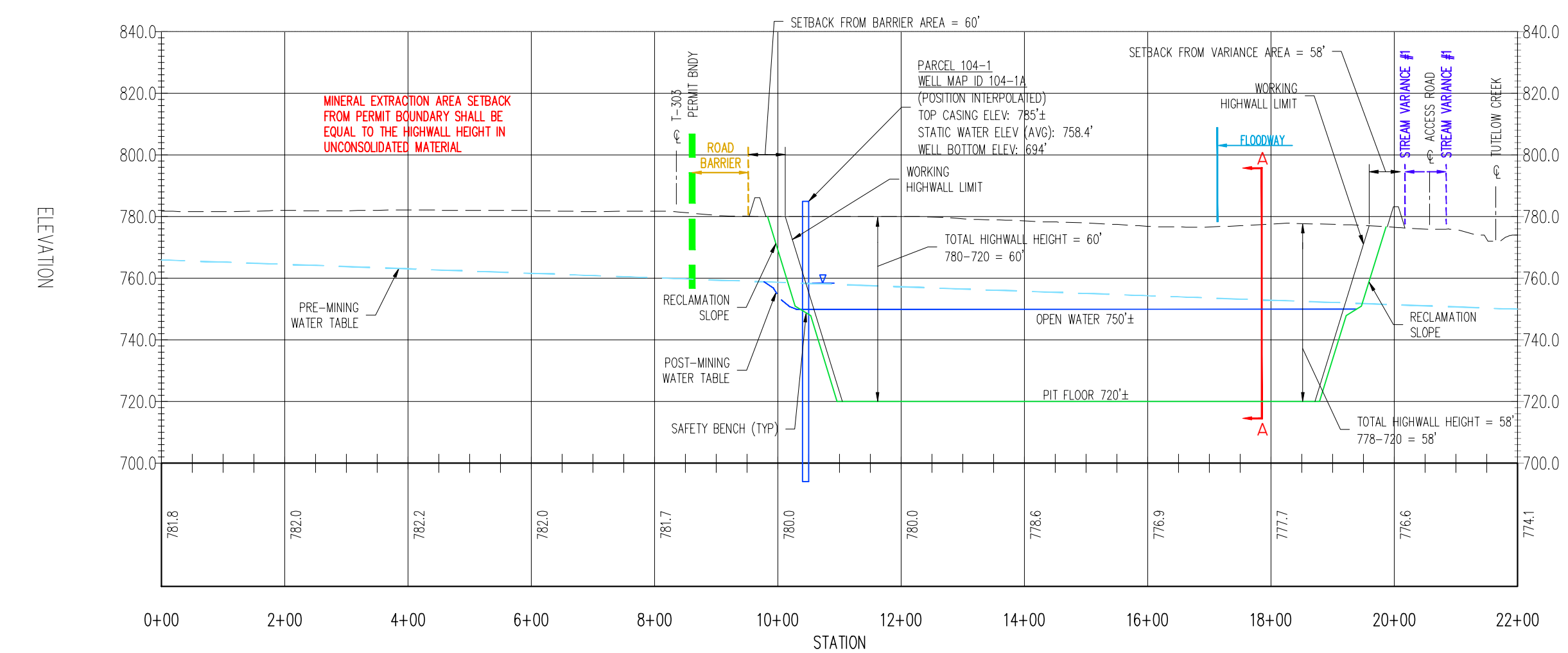
Section E-E'
