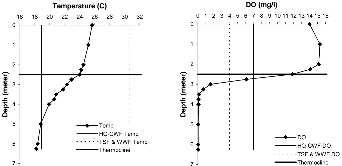
FIGURE 8. SPEEDWELL FORGE LAKE - WATER CHEMISTRY Temperature and Dissolved Oxygen Profiles - Dam DEP August 29, 1997
