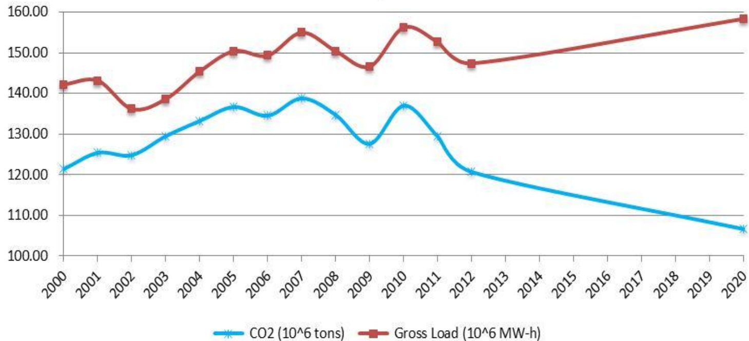
Carbon dioxide emission trends 2000-2020 from EGUs located in Pennsylvania
