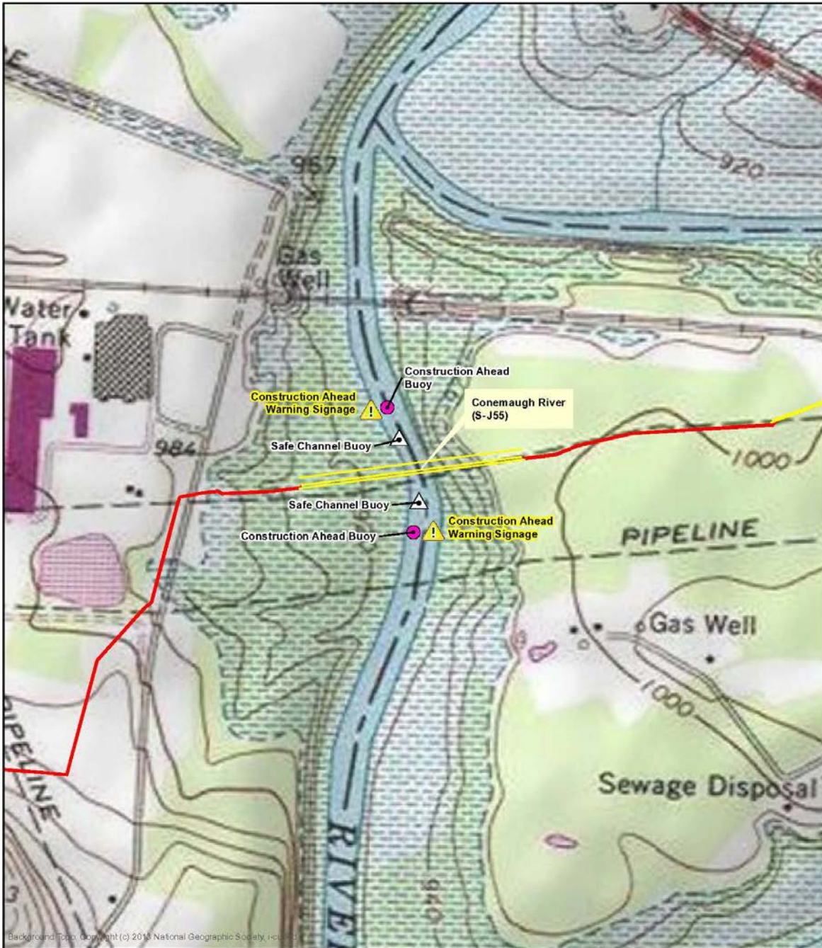
FIGURE 2 S-J55 CONEMAUGH RIVER ATON Plan Sunoco Mariner East Phase 2
