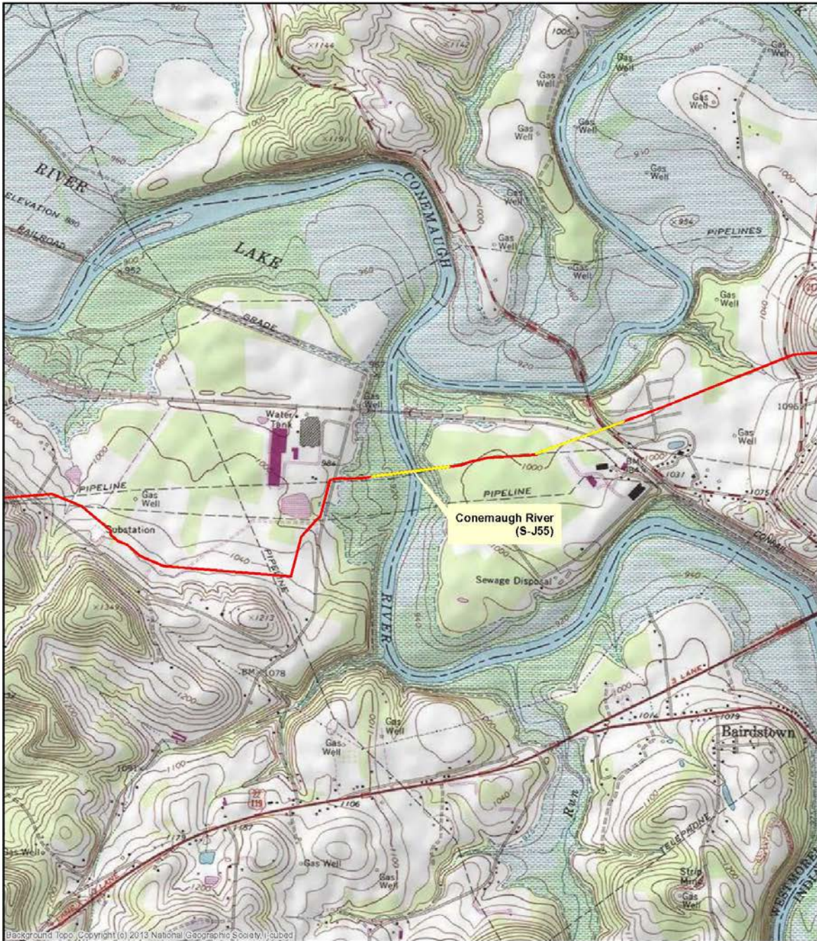
FIGURE 1 CONEMAUGH RIVER (S-J55) ATON Plan Sunoco Mariner East Phase 2
