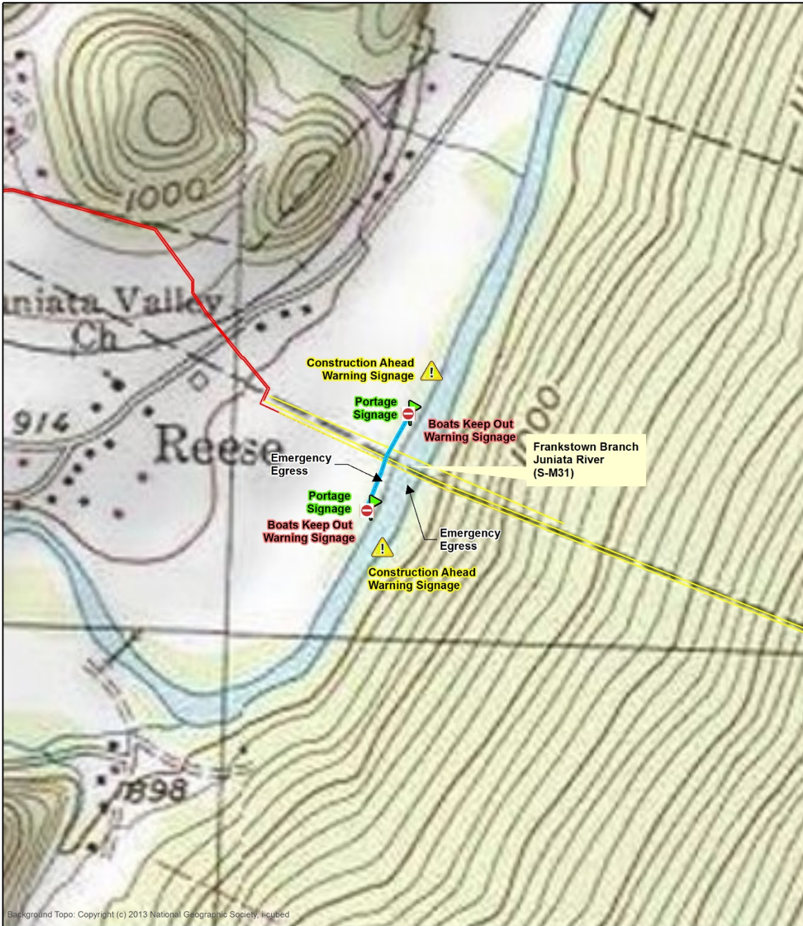
FIGURE 2 FRANKSTOWN BRANCH JUNIATA RIVER (S-M31) ATON Plan Sunoco Mariner East Phase 2
