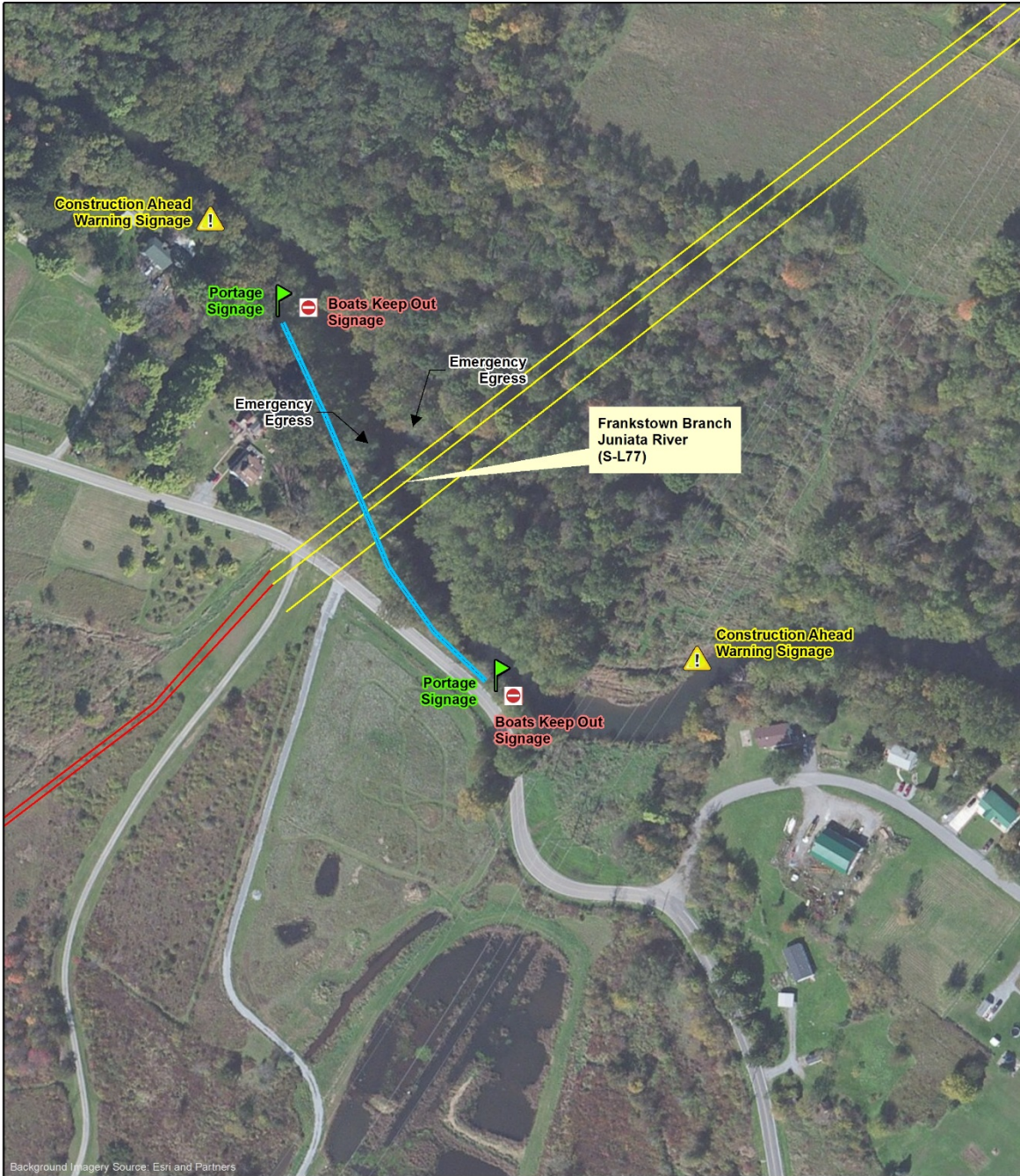
FIGURE 3 FRANKSTOWN BRANCH JUNIATA RIVER (S-L77) ATON Plan Sunoco Mariner East Phase 2
