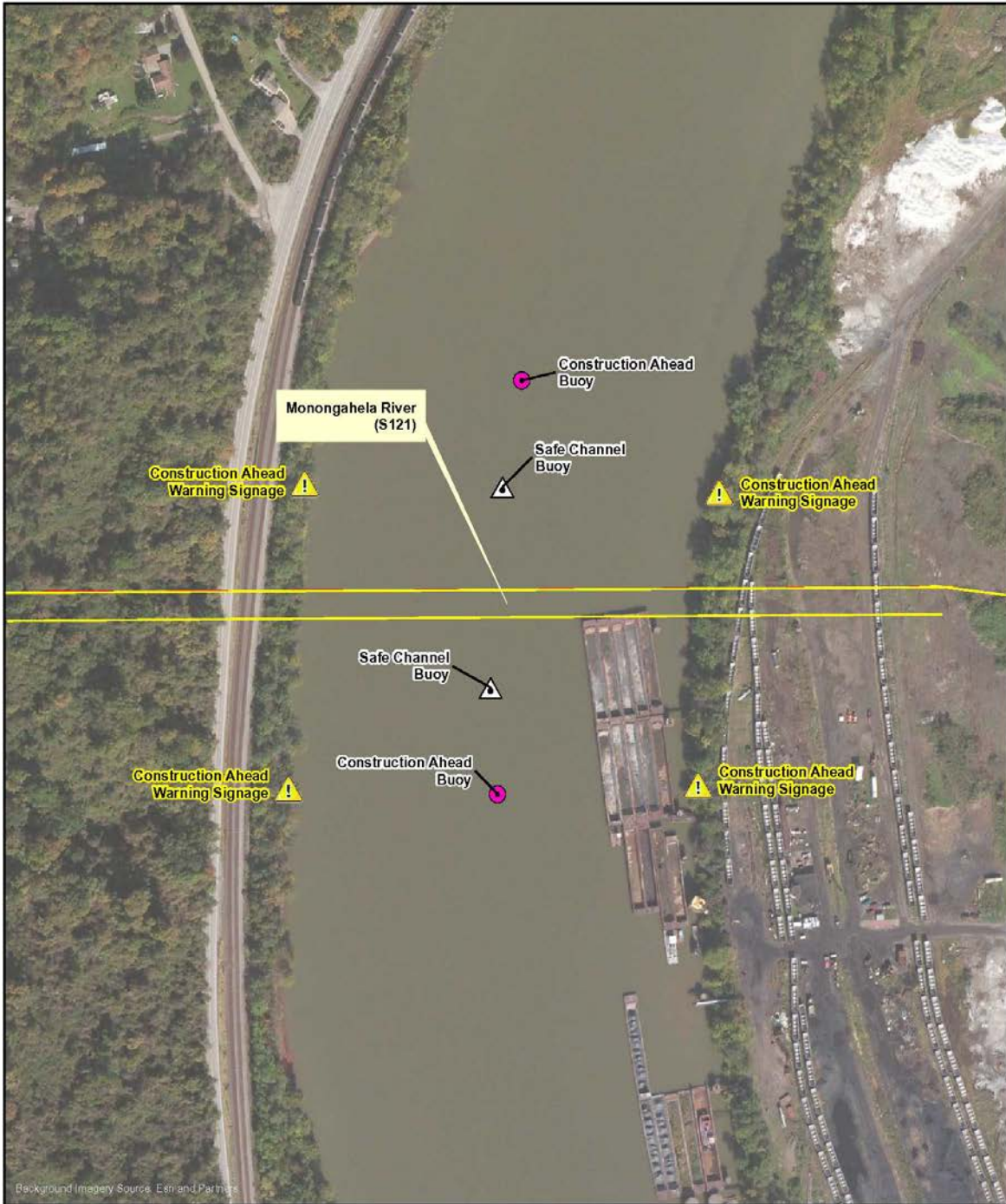
FIGURE 3 MONONGAHELA RIVER (S121) ATON Plan Sunoco Mariner East Phase 2
