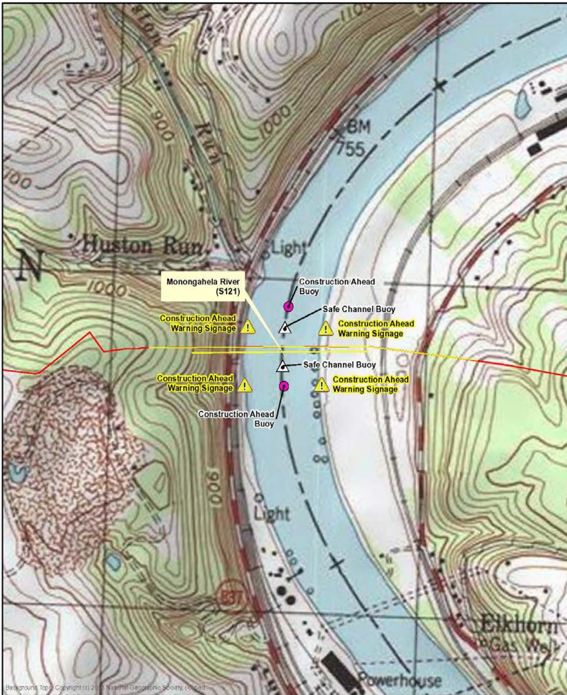
FIGURE 2 MONONGAHELA RIVER (S121) ATON Plan Sunoco Mariner East Phase 2
