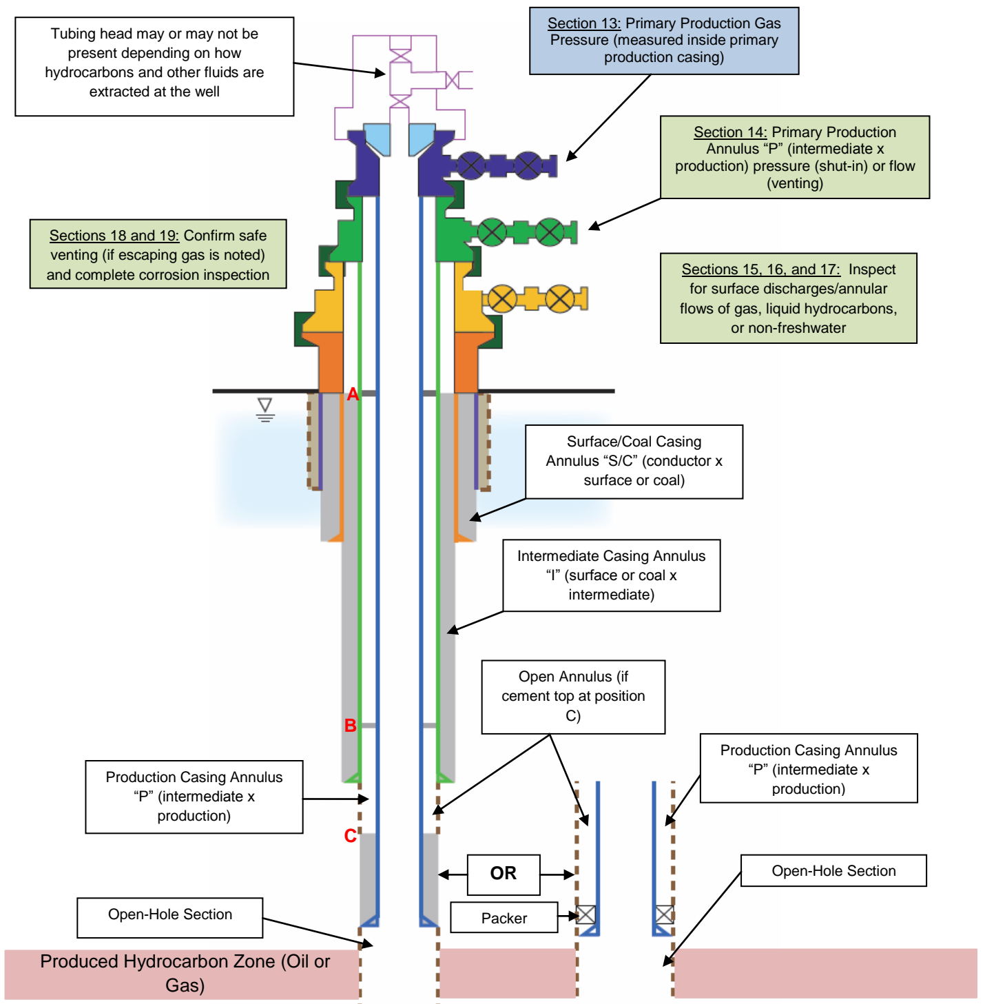
Figure 4 – Schematic representing a typical “MULTI-STRING” OPEN-HOLE COMPLETION WITH NO ANNULAR PRODUCTION (OIL OR GAS). The purple casing string represents the conductor pipe, the orange casing string represents the surface or coal protective casing, the green casing string represents the intermediate casing, and the blue casing string represents the production casing. If the well is only equipped with production and surface/coal casing, the “P” annulus is that annulus defined by those two casing strings. The annulus defined by the intermediate casing and surface casing is designated “I.” If multiple intermediate strings are utilized, the deepest is designated “I;” the second deepest, “I1;” and so forth. The annulus defined by the surface casing and conductor pipe is designated “S/C.” If multiple surface or coal protective strings are utilized, the deepest is designated “S/C;” the second deepest, “S/C1;” and so forth. Three different possible cement top positions are indicated as A, B, and C. A and B are for scenarios where the cement is circulated to the surface and inside of the intermediate string but not to the surface, respectively. C is for scenarios where the cement top is left below the intermediate shoe. The production casing may also be set on a packer as indicated to the left in the schematic. Inspection elements for gas wells only are indicated in blue. Those required for both oil and gas wells are indicated in green.
