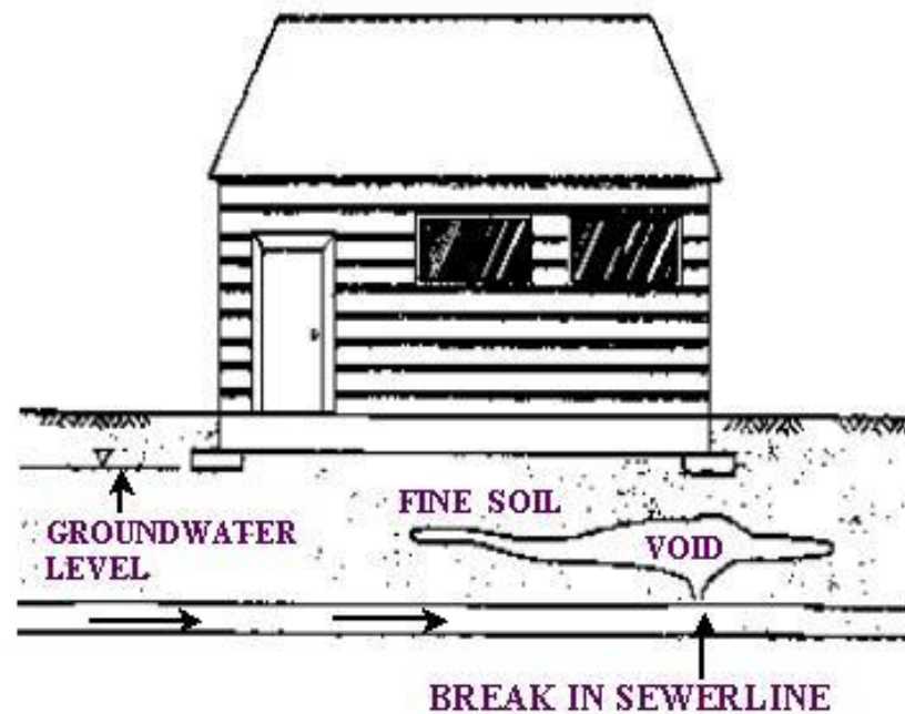
Void Created by Piping of Soil into Broken Sewer
