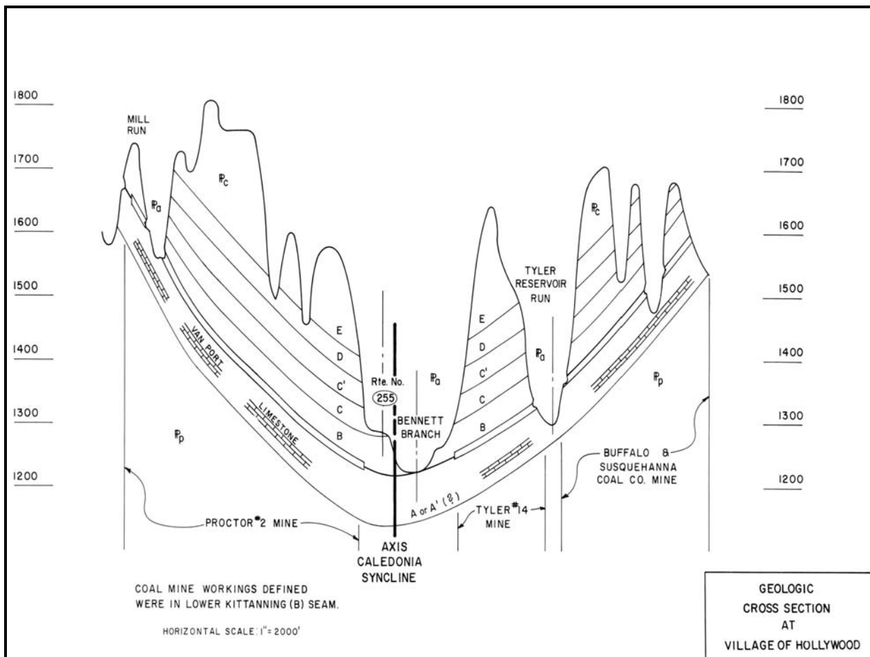
Figure 5. Cross section across the Bennett Branch stream valley near the Village of Hollywood (Source: Berger).
