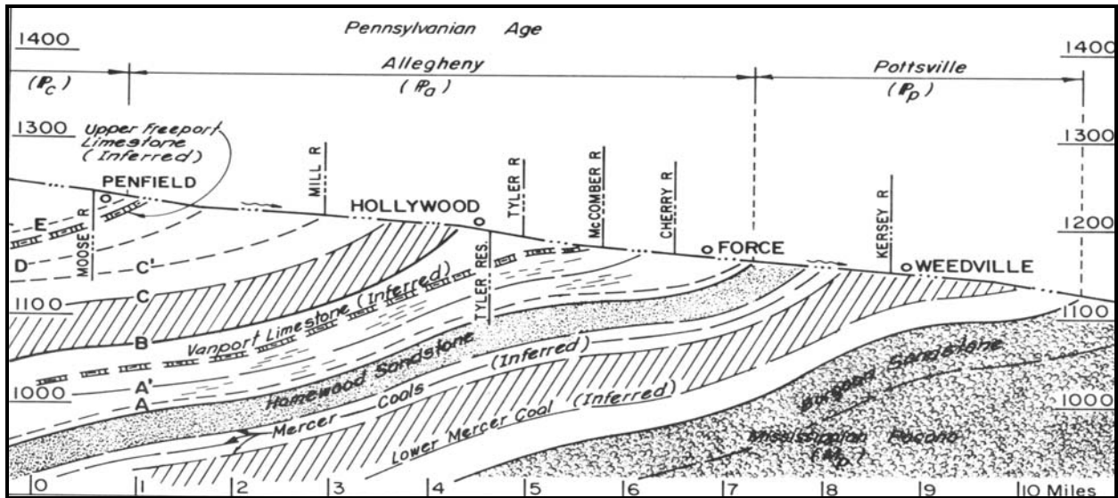
Figure 6. Profile along the axis of the Caledonia Syncline showing the plunge in the opposite direction of the stream flow (Source: Berger).
