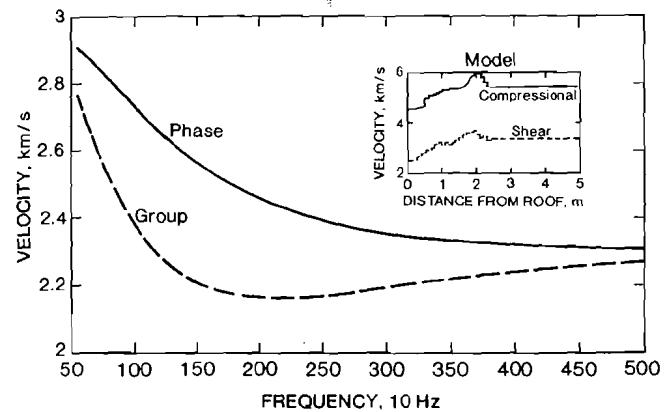
Figure 10.—Rayleigh wave dispersion for stressed metal mine roof model.
