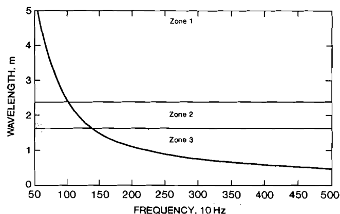
Figure 13.—Wavelength as function of frequency for stressed metal mine roof model.
