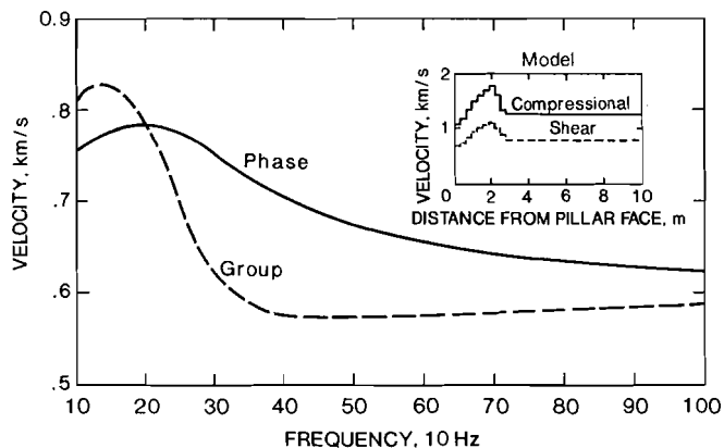
Figure 6.—Rayleigh wave dispersion for stressed coal pillar model.
