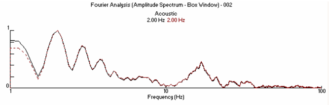
Figure 3. White Test 1 Comparison of 0 and 3 Feet.
