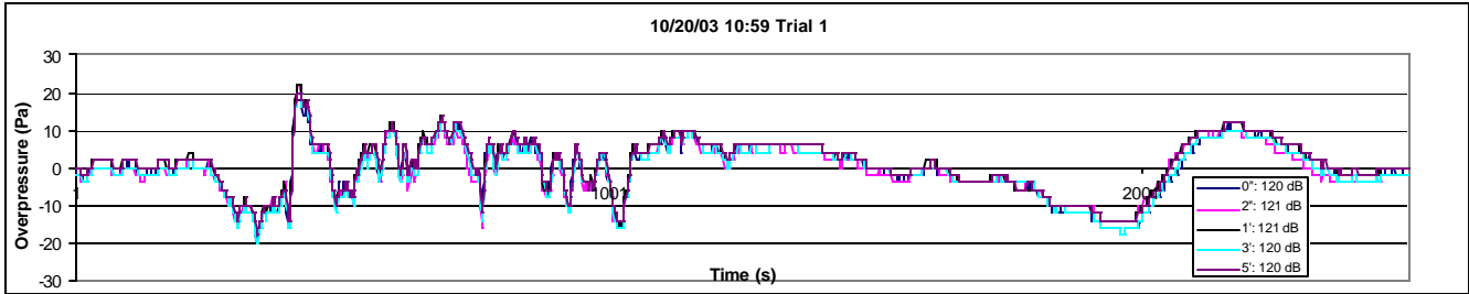
Figure 16. OSM Test 4 Waveform Comparison.
