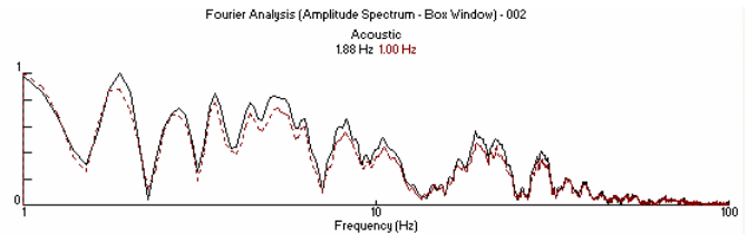
Figure 7. White Test 3 Comparison of 0 and 3 Feet.
