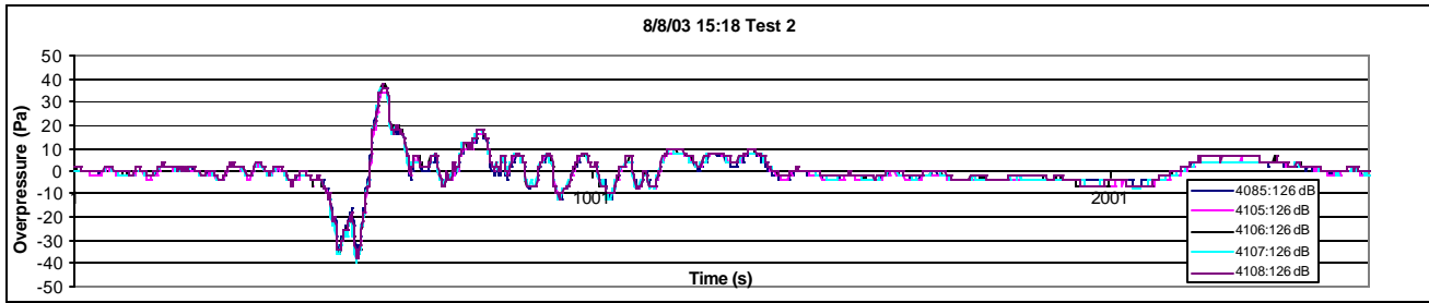
Figure 14. OSM Test 2 Waveform Comparison.
