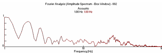
Figure 10. White Test 5 Comparison of 1 and 3 Feet.
