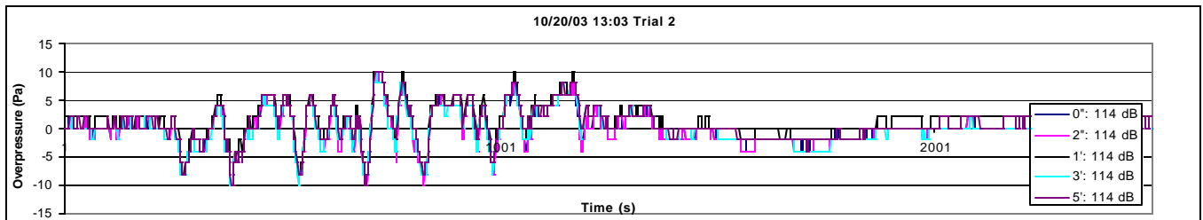
Figure 15. OSM Test 3 Waveform Comparison.
