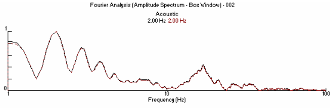
Figure 2. White Test 1 Comparison of 1 and 3 Feet.
