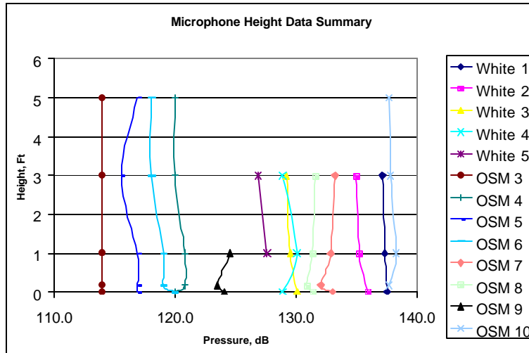
Figure 23. Data Summary of White and OSM Tests.
