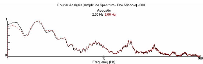
Figure 5. White Test 2 Comparison of 0 and 3 Feet.
