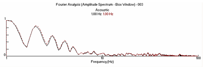
Figure 9. White Test 4 Comparison of 0 and 3 Feet.
