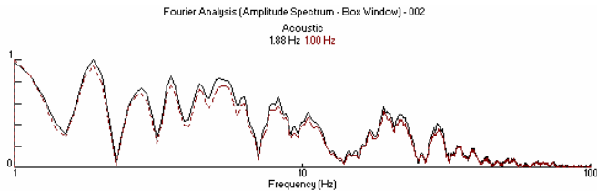
Figure 6. White Test 3 Comparison of 1 and 3 Feet.
