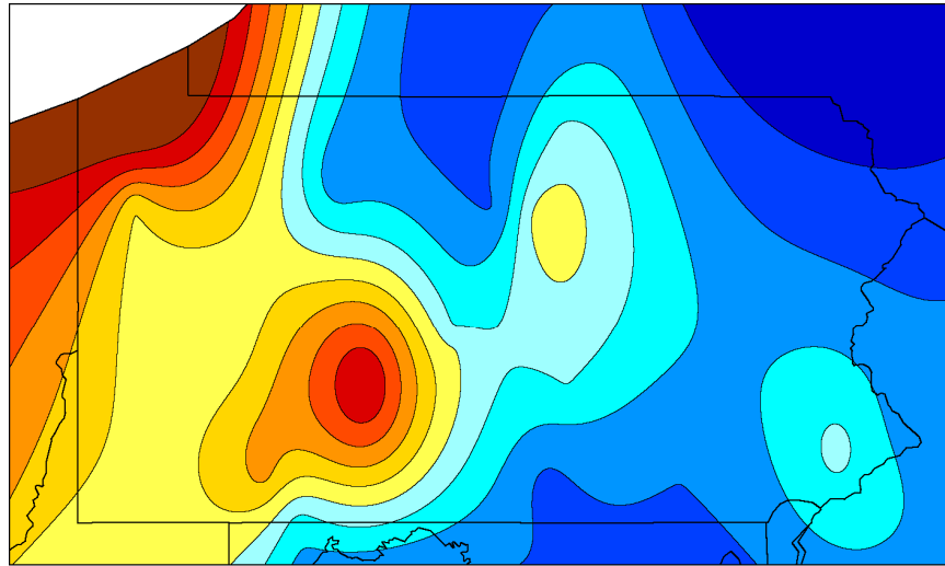
Annual Calcium Concentration: 2006
