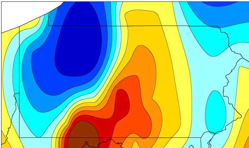
Growing Season Precipitation: 2006
