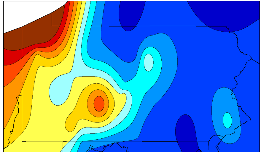
Dormant Season Calcium Concentration: 2006
