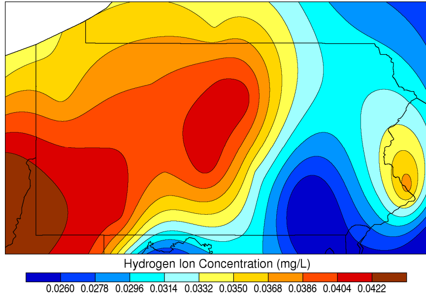
Annual Hydrogen Ion Concentration: 2006
