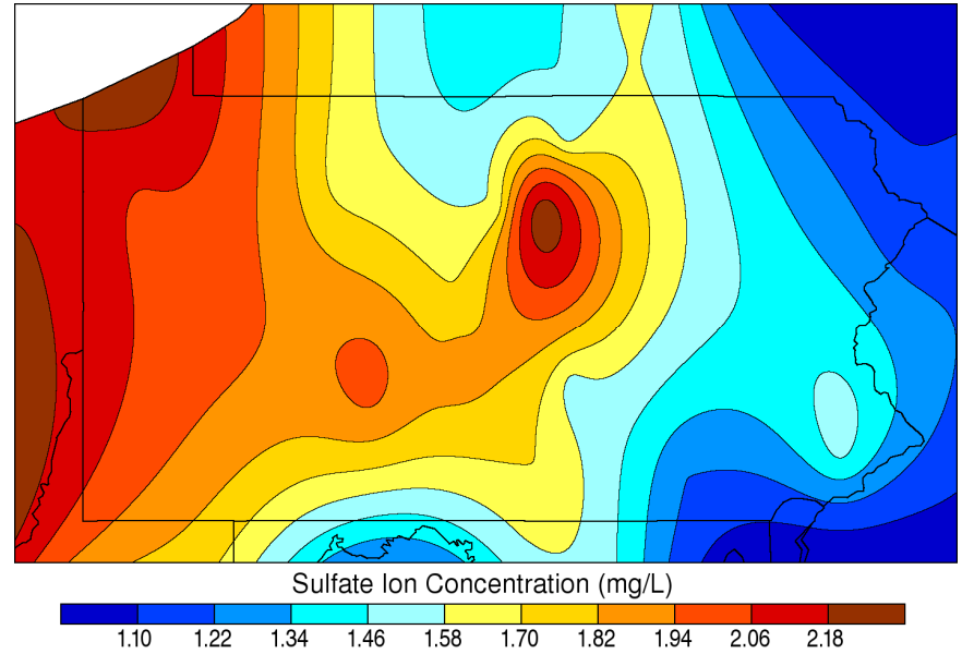
Dormant Season Sulfate Concentration: 2006
