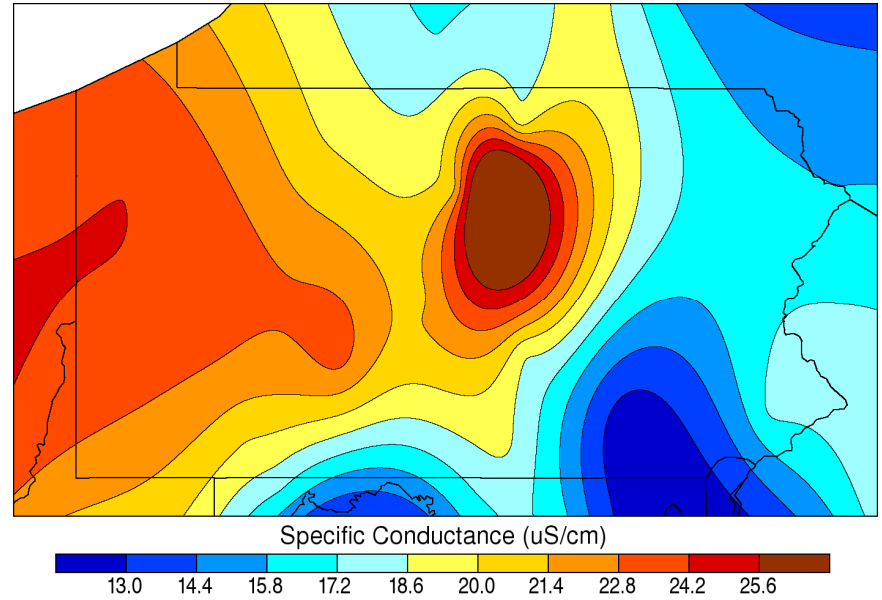
Dormant Season Specific Conductance: 2006
