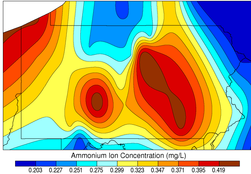
Annual Ammonium Concentration: 2006
