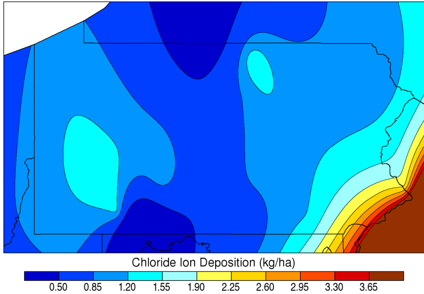
Growing Season Chloride Wet Deposition: 2006
