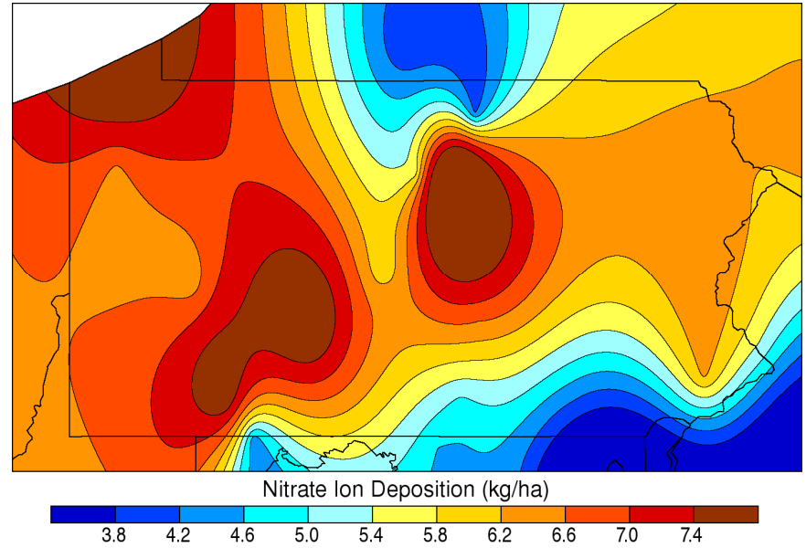
Dormant Season Nitrate Wet Deposition: 2006
