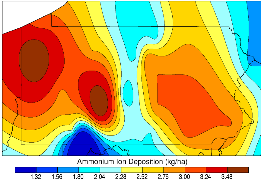
Growing Season Ammonium Wet Deposition: 2006
