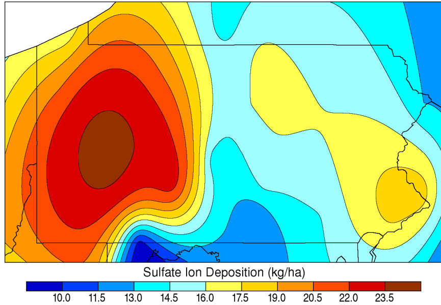
Growing Season Sulfate Wet Deposition: 2006
