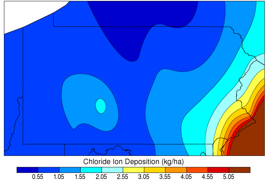
Dormant Season Chloride Wet Deposition: 2006
