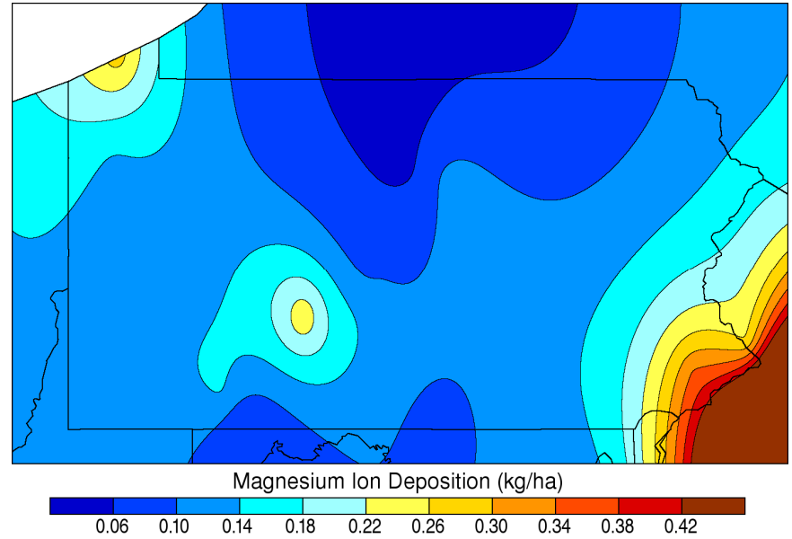
Dormant Season Magnesium Wet Deposition: 2006
