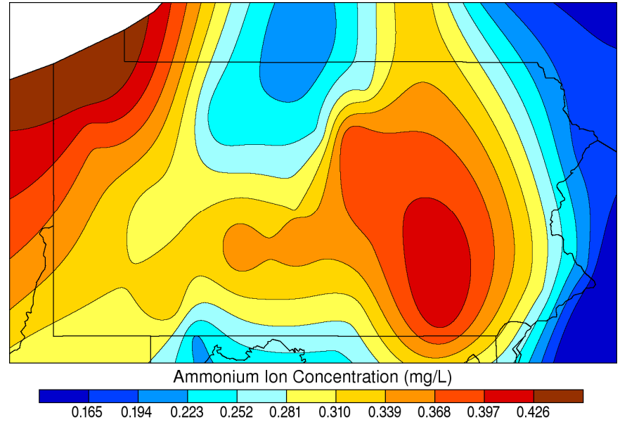
Dormant Season Ammonium Concentration: 2006
