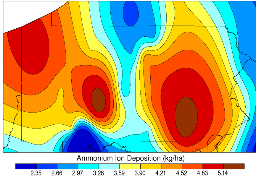
Annual Ammonium Wet Deposition: 2006
