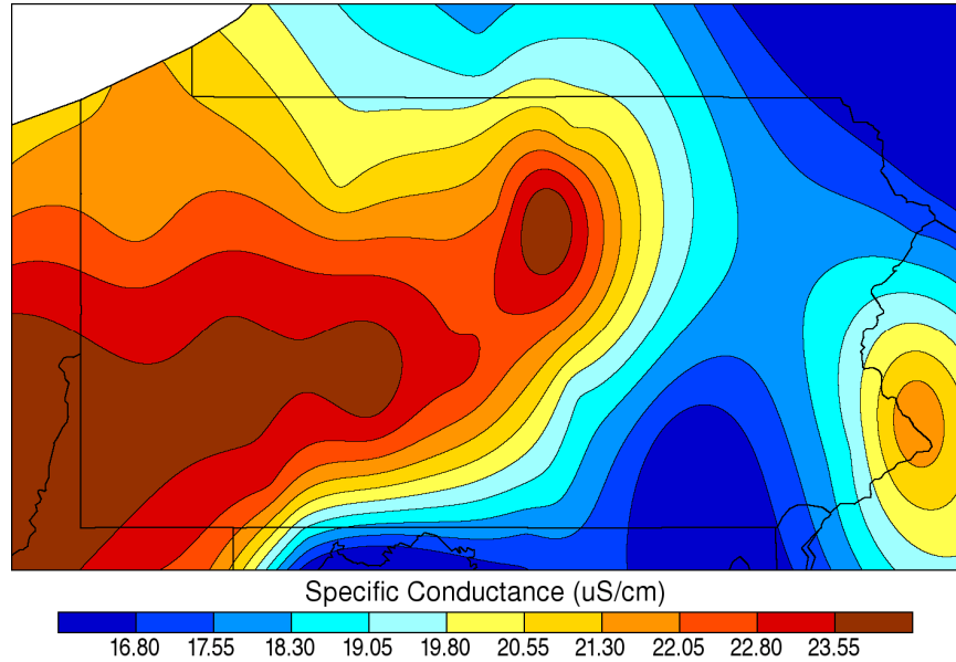
Annual Specific Conductance: 2006
