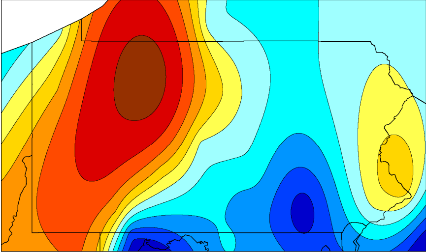
Annual Hydrogen Ion Wet Deposition: 2006
