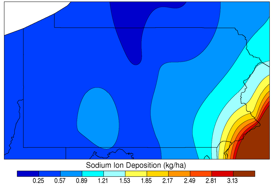
Dormant Season Sodium Wet Deposition: 2006
