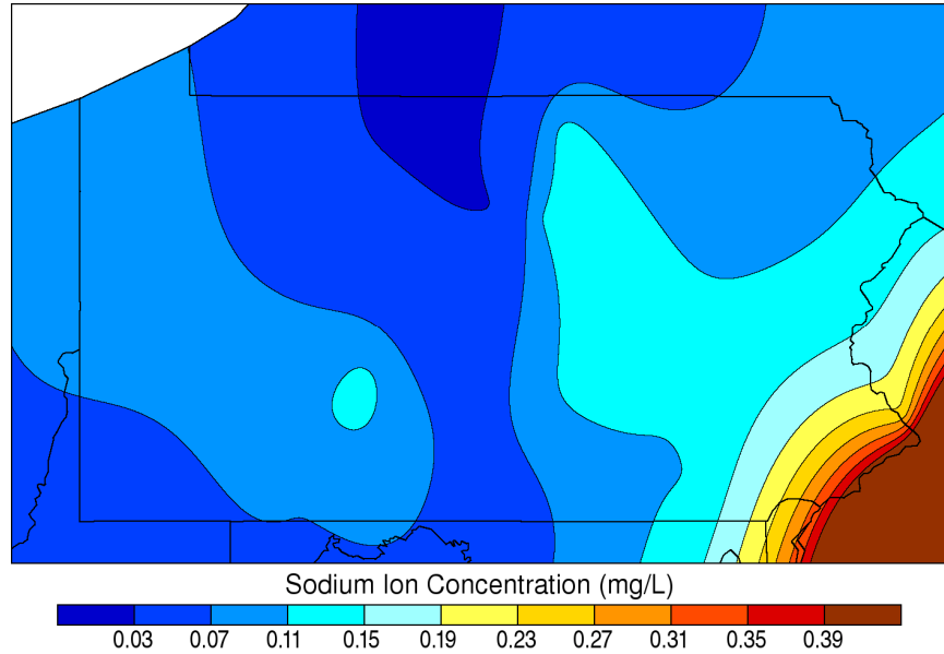
Annual Sodium Concentration: 2006
