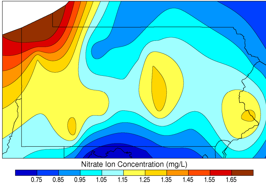
Growing Season Nitrate Concentration: 2006
