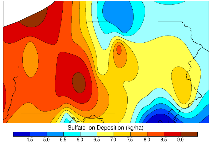
Dormant Season Sulfate Wet Deposition: 2006
