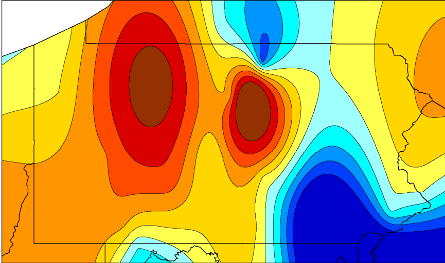
Dormant Season Hydrogen Ion Wet Deposition: 2006
