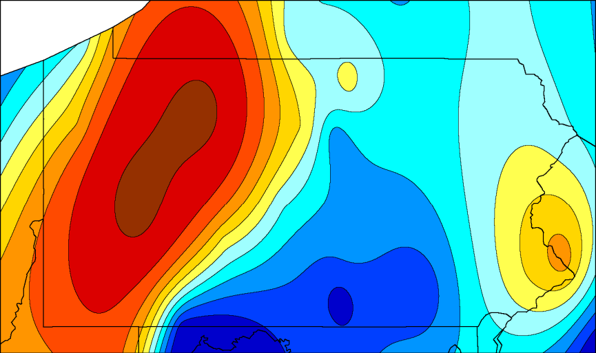
Growing Season Hydrogen Ion Wet Deposition: 2006
