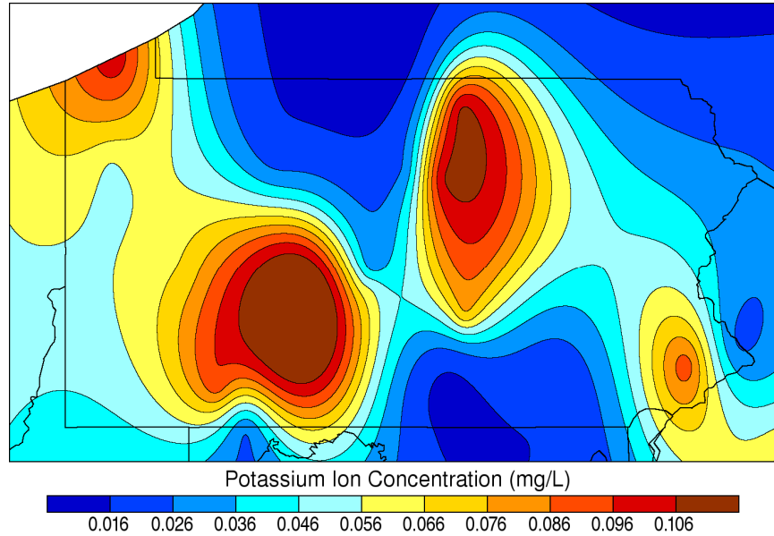
Annual Potassium Concentration: 2006
