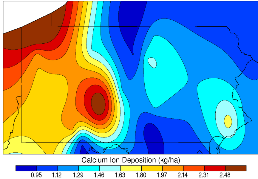
Annual Calcium Wet Deposition: 2006
