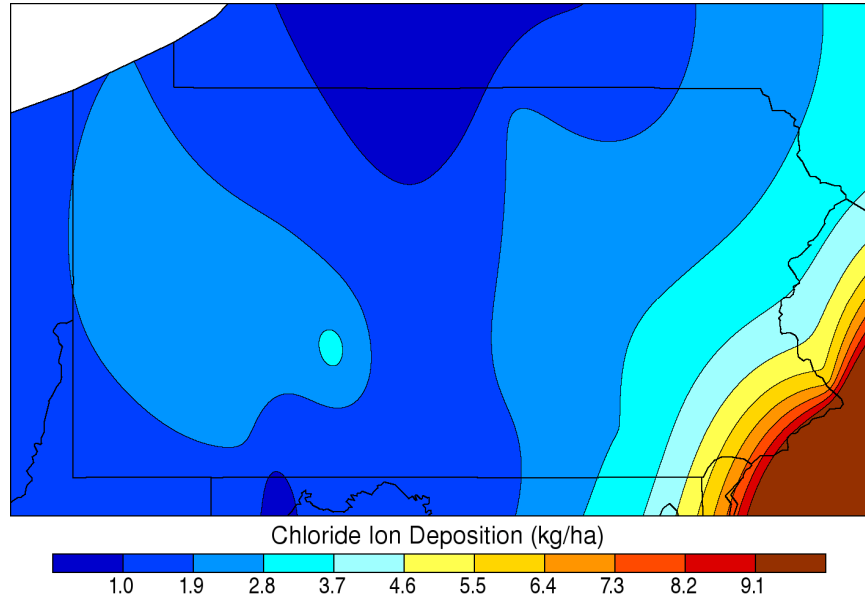
Annual Chloride Wet Deposition: 2006
