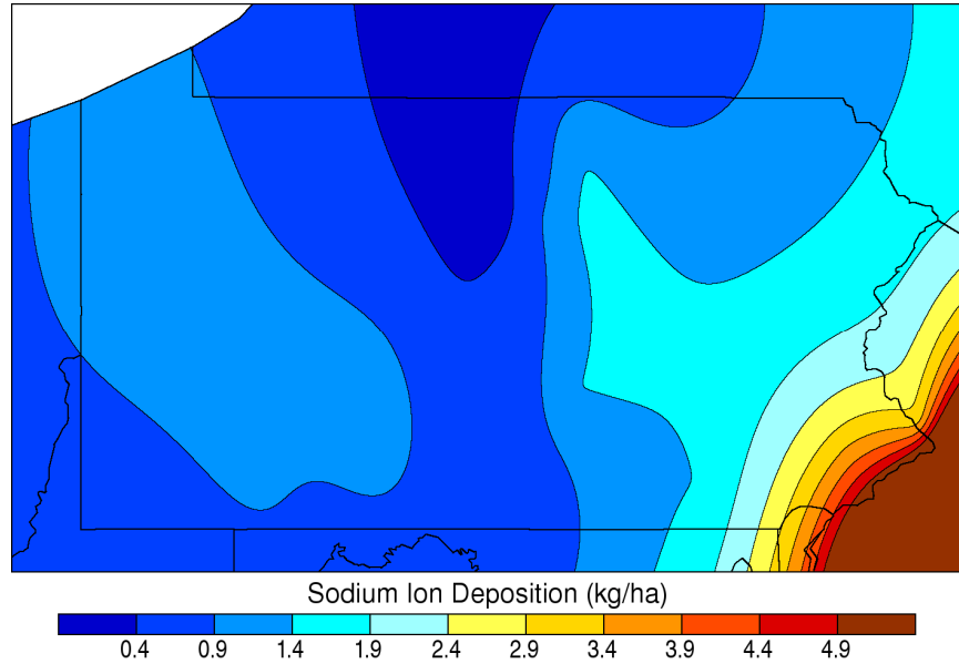
Annual Sodium Wet Deposition: 2006
