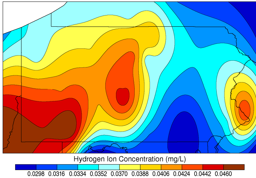
Growing Season Hydrogen Ion Concentration: 2006
