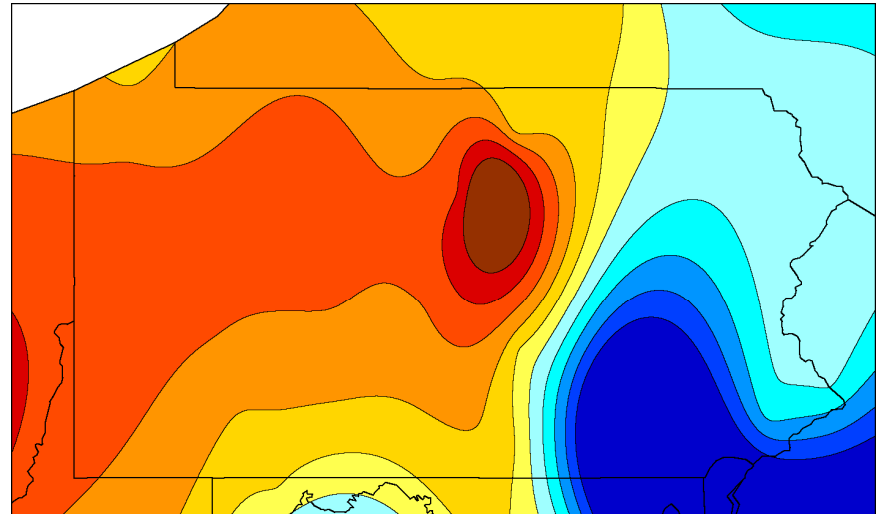
Dormant Season pH: 2006
