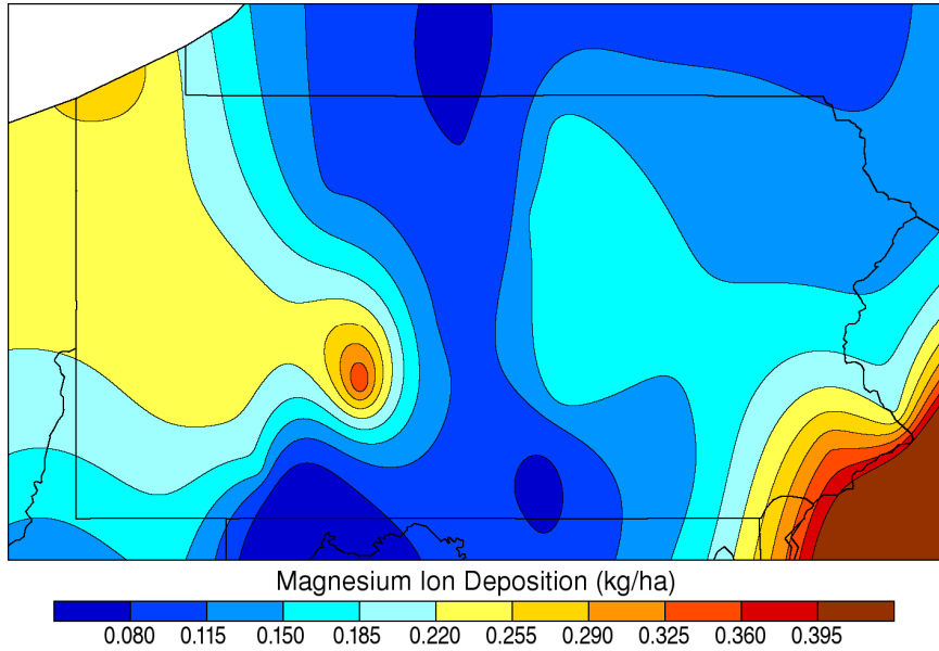
Growing Season Magnesium Wet Deposition: 2006
