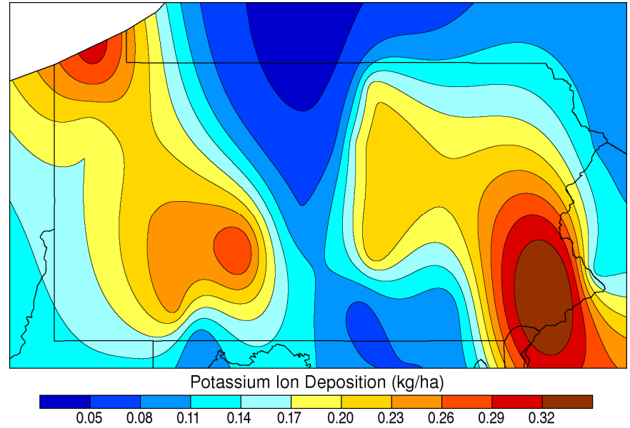
Dormant Season Potassium Wet Deposition: 2006
