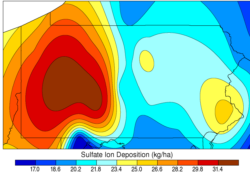
Annual Sulfate Wet Deposition: 2006
