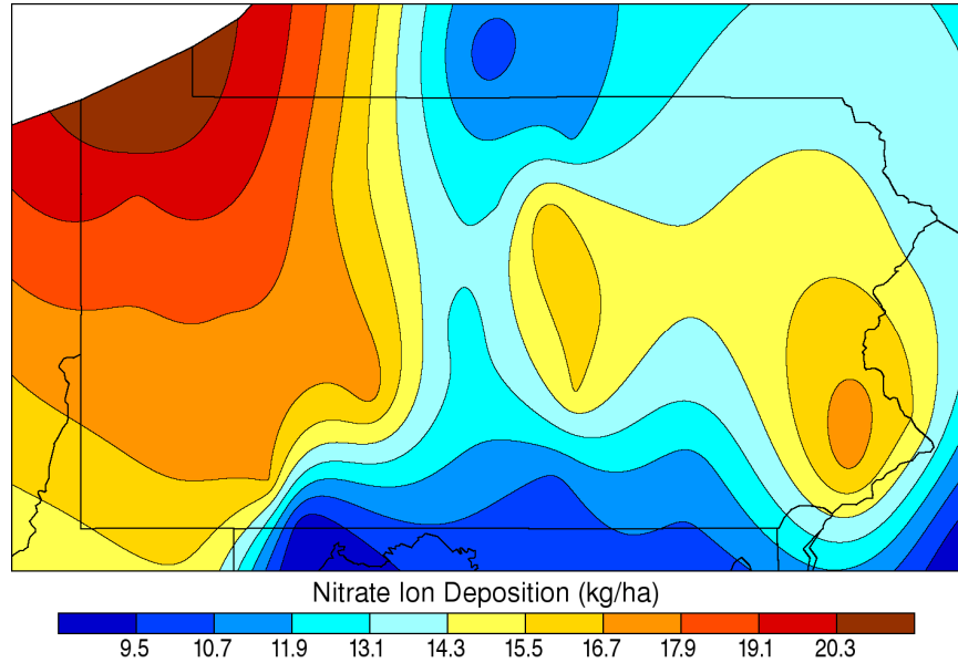
Annual Nitrate Wet Deposition: 2006
