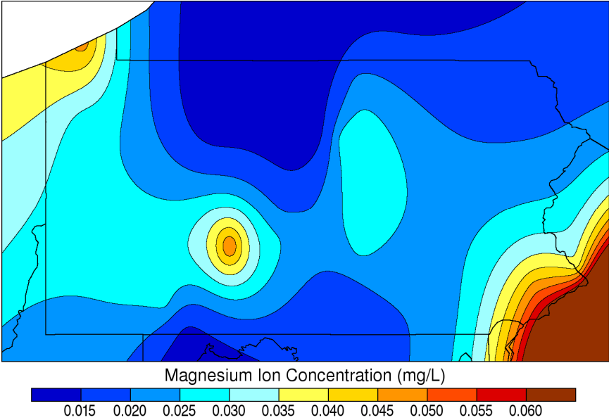
Annual Magnesium Concentration: 2006
