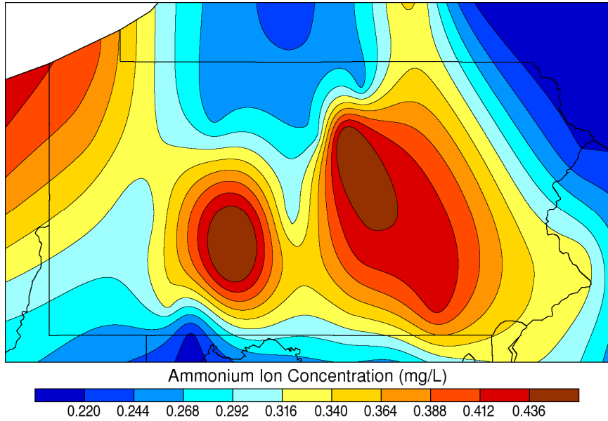
Growing Season Ammonium Concentration: 2006
