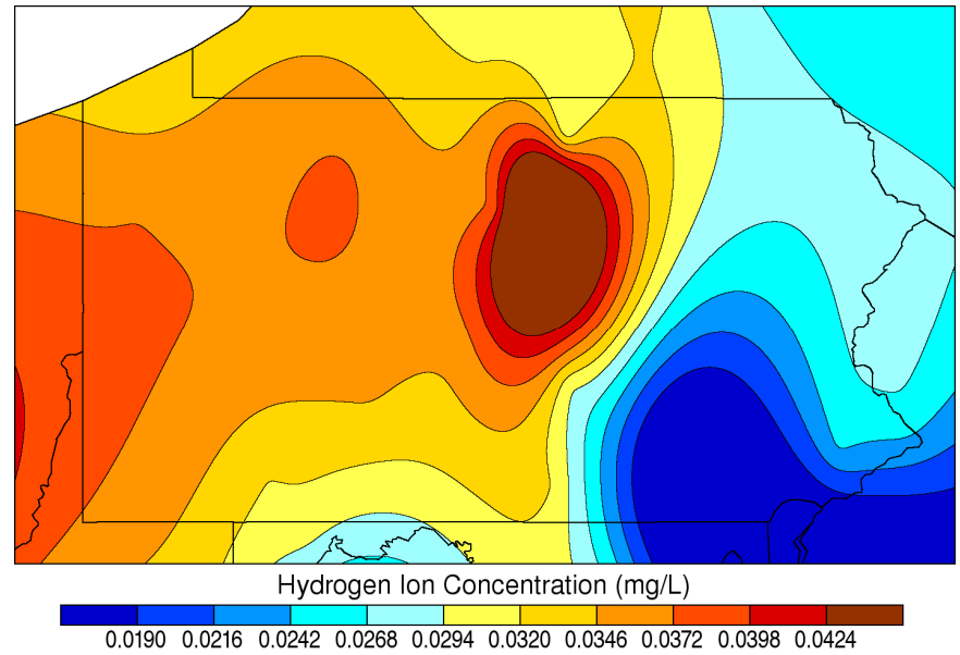
Dormant Season Hydrogen Ion Concentration: 2006
