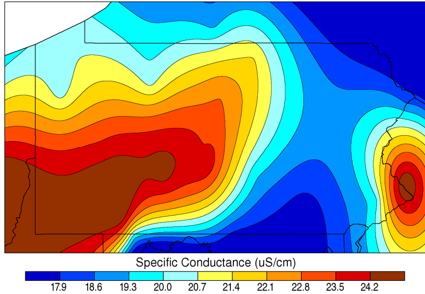
Growing Season Specific Conductance: 2006
