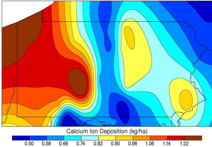
Growing Season Calcium Wet Deposition: 2006
