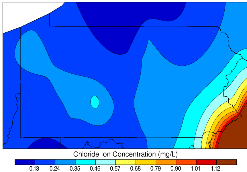
Dormant Season Chloride Concentration: 2006
