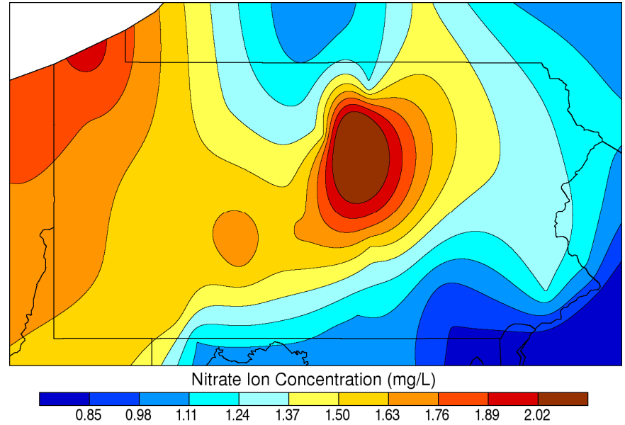
Dormant Season Nitrate Concentration: 2006
