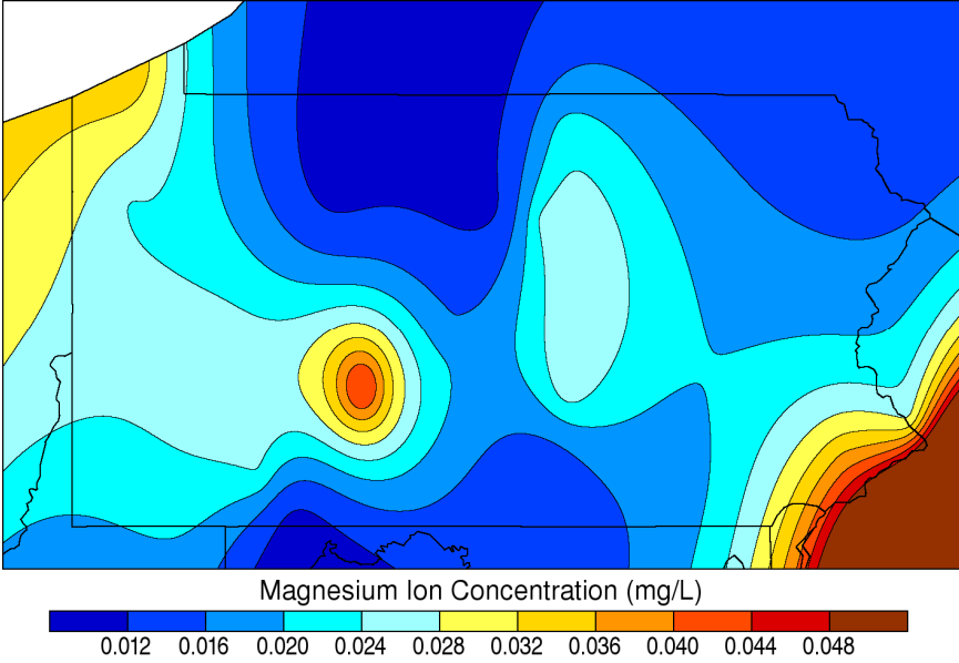
Growing Season Magnesium Concentration: 2006
