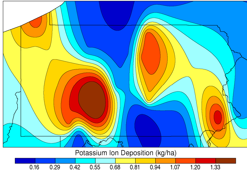
Annual Potassium Wet Deposition: 2006
