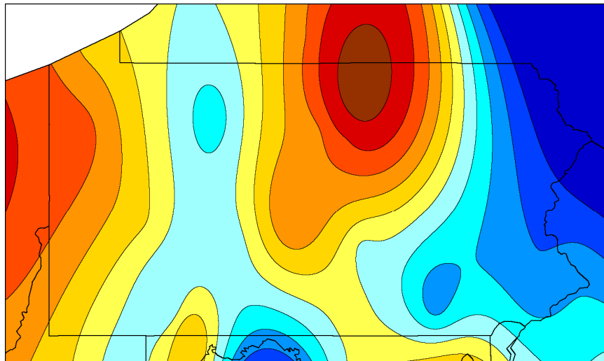
Dormant Season Precipitation: 2006
