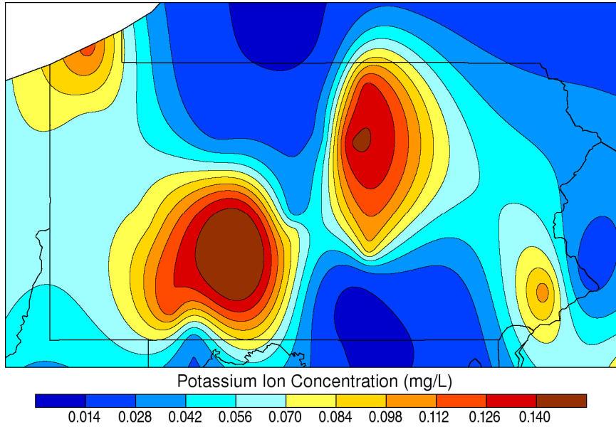
Growing Season Potassium Concentration: 2006
