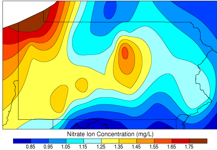
Annual Nitrate Concentration: 2006
