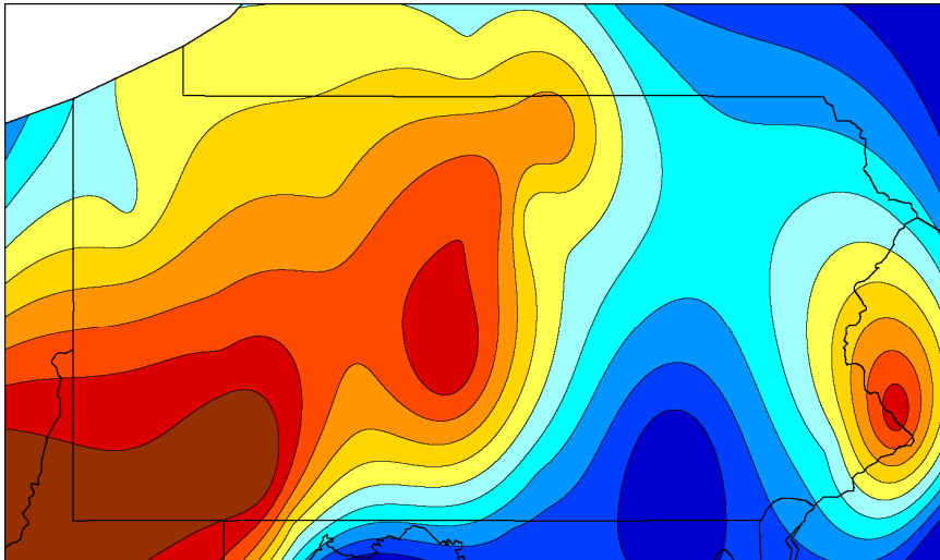
Growing Season pH: 2006
