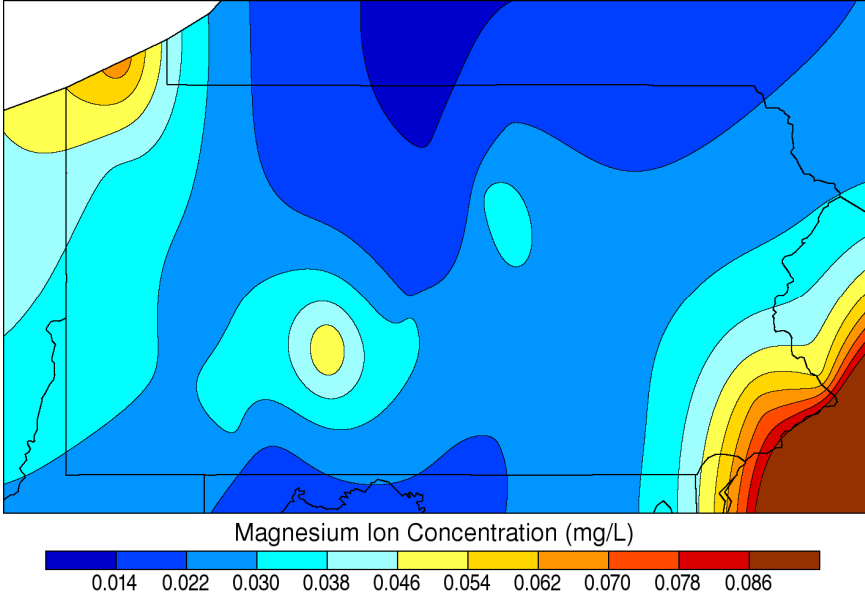
Dormant Season Magnesium Concentration: 2006
