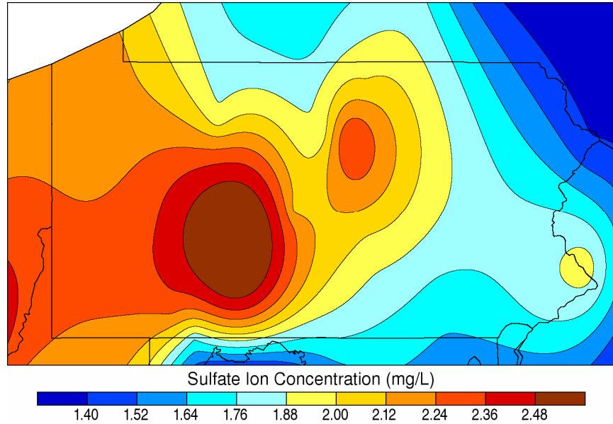
Annual Sulfate Concentration: 2006
