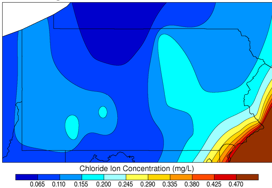
Growing Season Chloride Concentration: 2006
