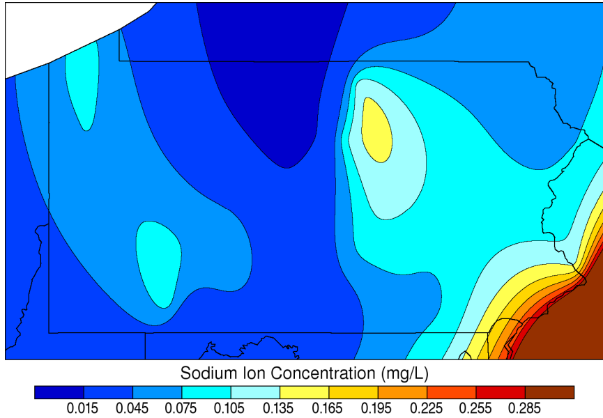
Growing Season Sodium Concentration: 2006
