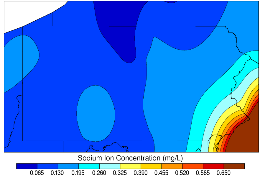
Dormant Season Sodium Concentration: 2006
