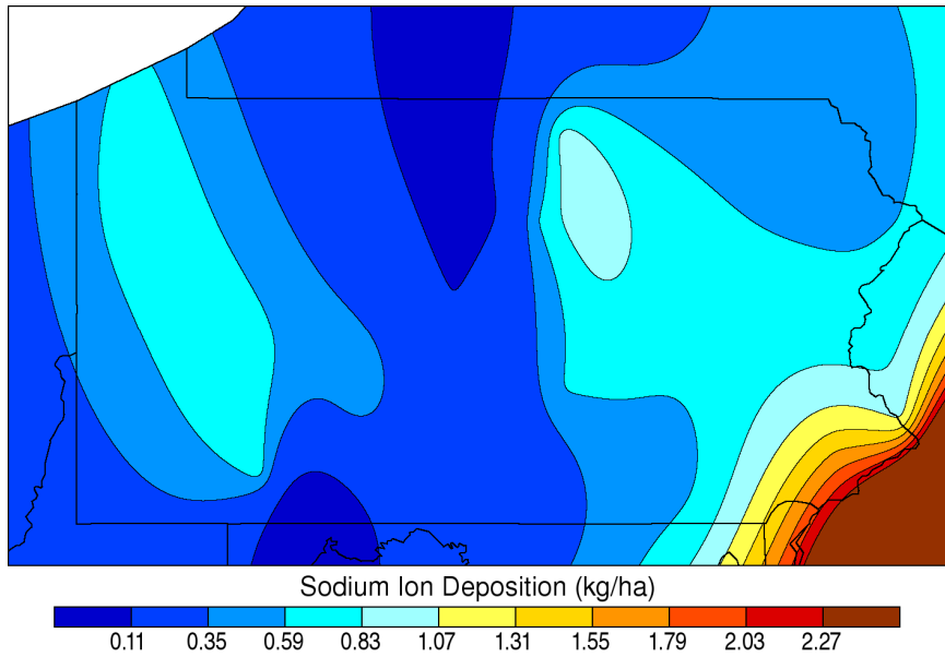
Growing Season Sodium Wet Deposition: 2006
