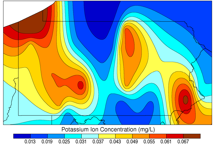
Dormant Season Potassium Concentration: 2006
