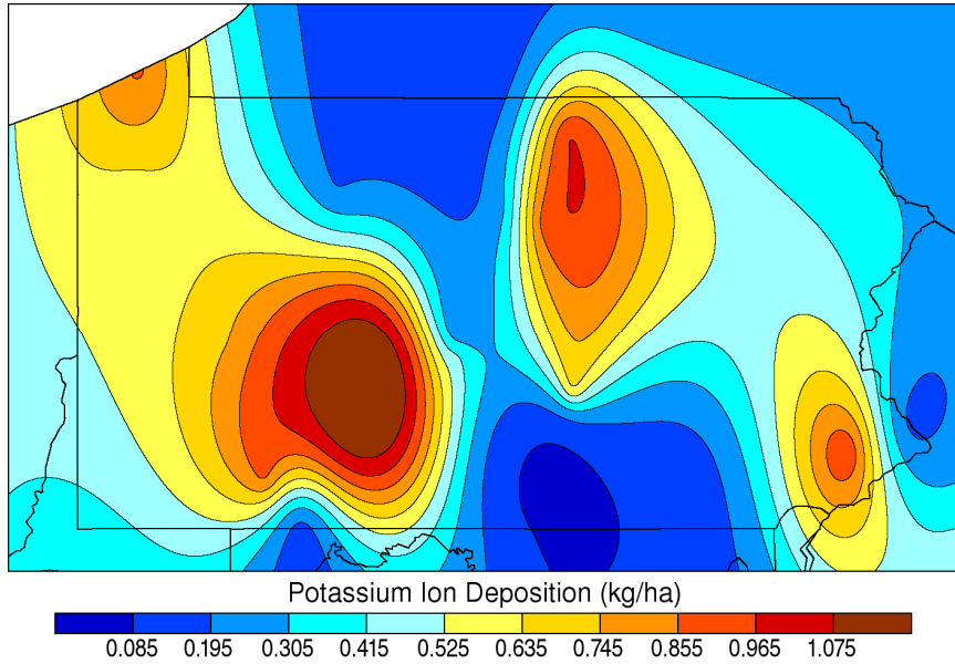
Growing Season Potassium Wet Deposition: 2006
