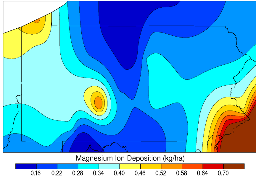
Annual Magnesium Wet Deposition: 2006
