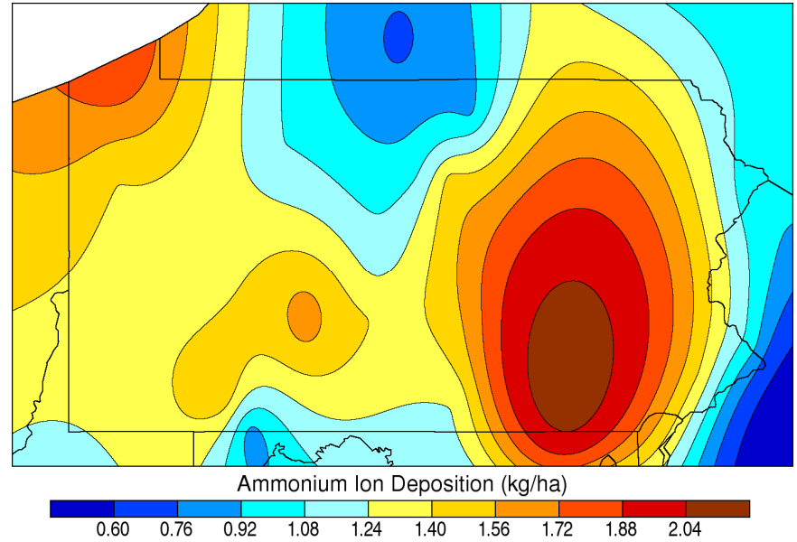
Dormant Season Ammonium Wet Deposition: 2006
