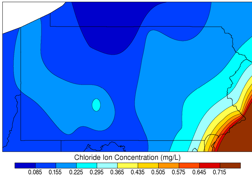
Annual Chloride Concentration: 2006
