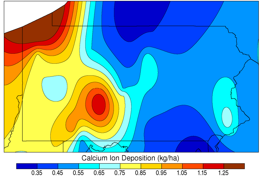
Dormant Season Calcium Wet Deposition: 2006
