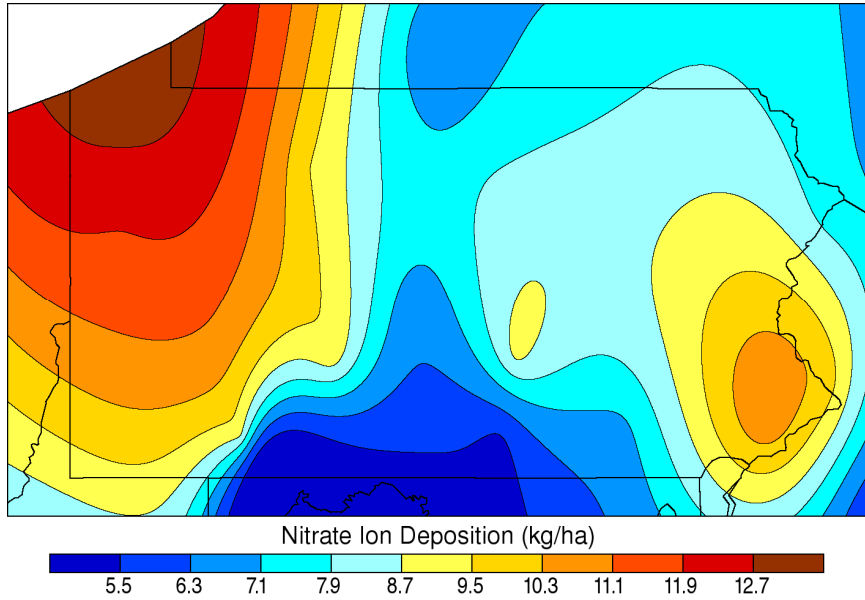
Growing Season Nitrate Wet Deposition: 2006
