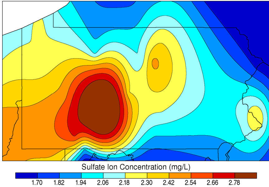
Growing Season Sulfate Concentration: 2006
