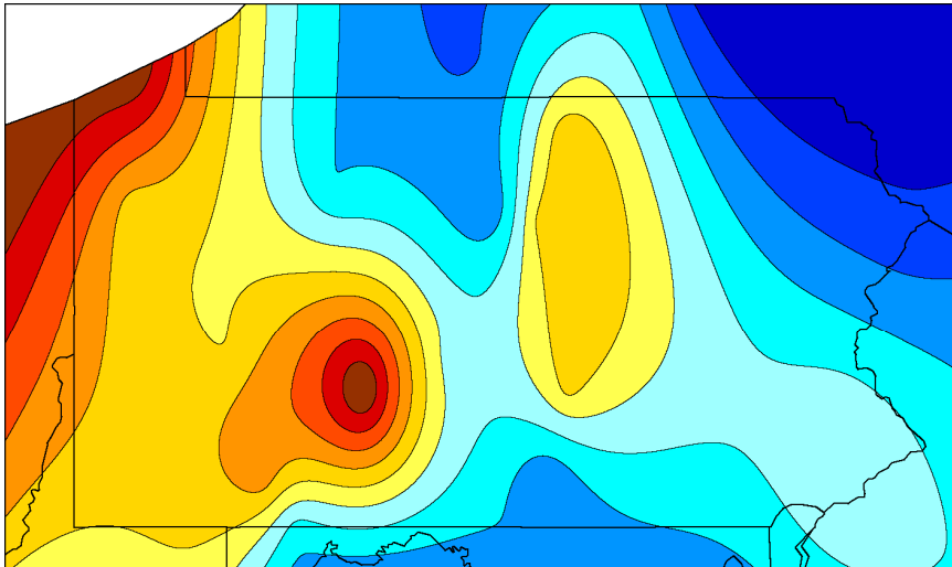
Growing Season Calcium Concentration: 2006
