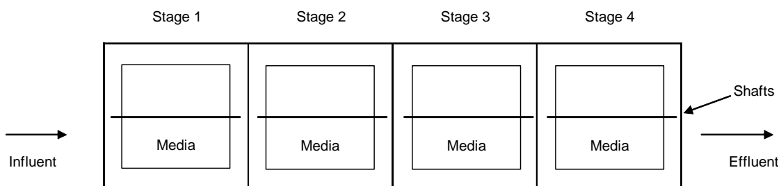
Figure 1.9 Four Stages with Four Shafts and Flow Parallel to the Shaft
