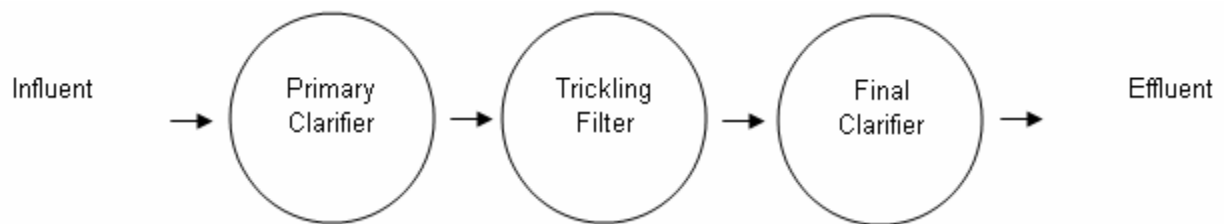
Figure 1.21 Single-Stage Trickling Filter Arrangement
