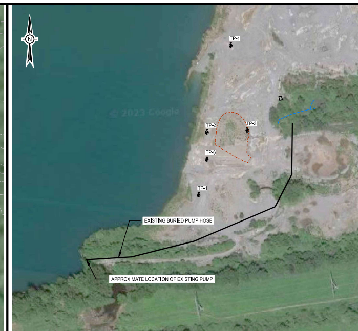
PUMPING LOCATION PLAN 0 200 400
