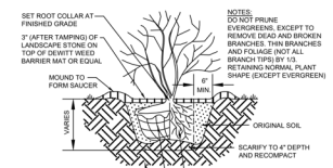
SHRUB PLANTING - SINGLE NOT TO SCALE
