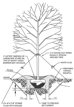
TREE PLANTING DETAIL NOT TO SCALE
